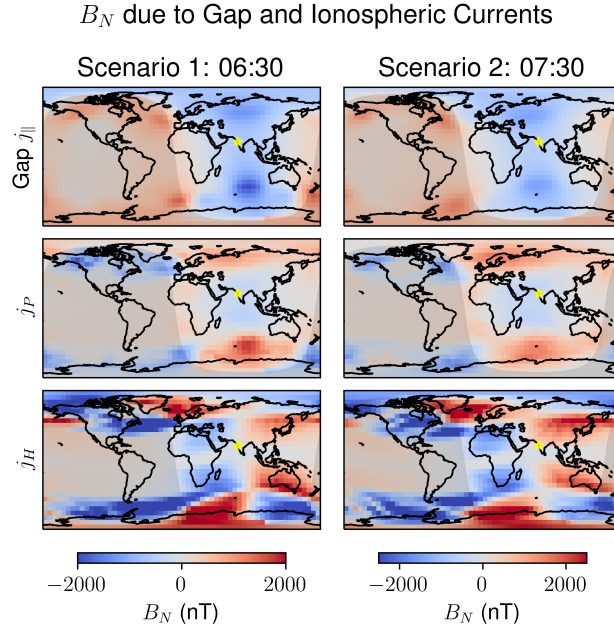
Figure 8. Comparison of heatmaps from Scenario 1 at 06:30 (UTC) and Scenario 2 at 07:30 (UTC), near the storm peak. These heatmaps are taken, unchanged, from Figures 6 and 7. Although the solar wind conditions are different, the similarities between the heatmaps are apparent.
