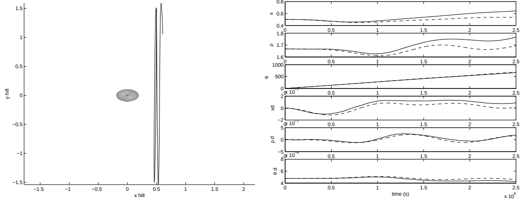
Figure 6.18: Orbit with Initial Offset of x = 0.5 km with Ellipsoidal Body with Radii 0.193, 0.105, and 0.105 km. Solid = Trajectory. Dashed = Trajectory Assuming a Spherical Body.
