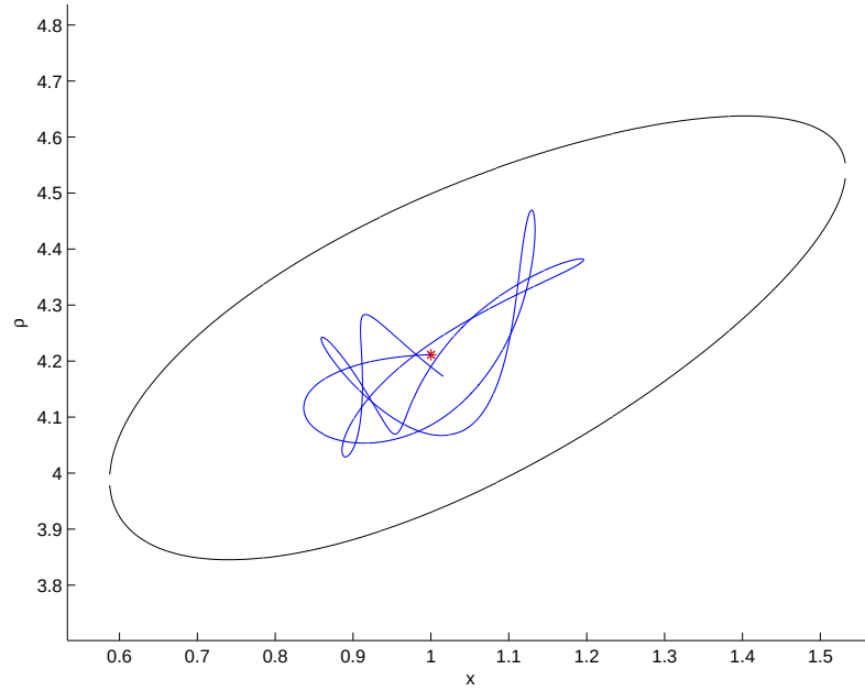
Figure 6.13: Stable Trajectory Plotted on Zero Velocity Curves. Blue = Trajectory. Black = Trajectory Zero velocity Curve. Red = Averaged Equilibrium Zero Velocity Curve.
