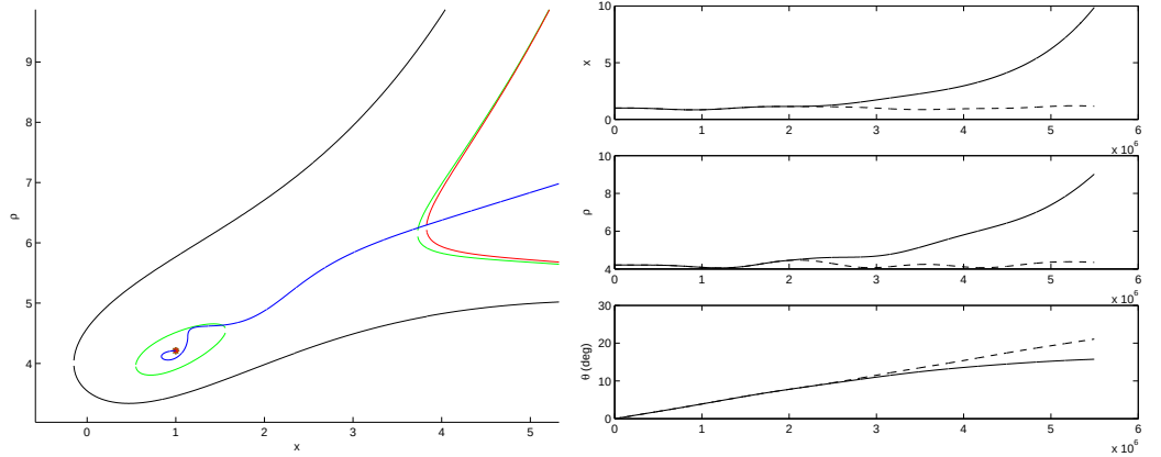
Figure 6.16: Unstable Trajectory in the Presence of an Outgassing Jet on Appropriate Zero Velocity Curve (Two Jet Passages). Blue = Trajectory. Black = Zero velocity Curve with Outgassing. Black = Zero velocity Curve without Outgassing. Shown with Position Components. Solid = Trajectory with Outgassing. Dashed = Trajectory Without Outgassing.
