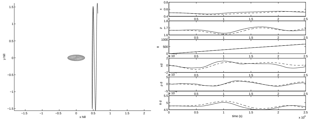
Figure 6.19: Orbit with Initial Offset of x = 0.5 km with Ellipsoidal Body with Radii 0.258, 0.091, and 0.091 km. Solid = Trajectory. Dashed = Trajectory Assuming a Spherical Body.
