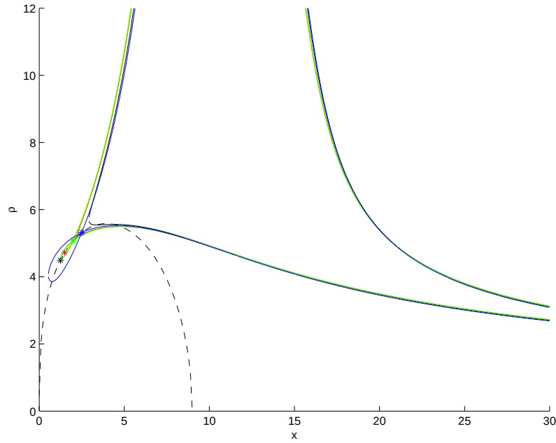
Figure 6.7: Zero Velocity Curves for Various Equilibrium Solutions. * = equilibrium solution at each C Energy Level. Dashed = Circular Orbit Equilibrium Solutions Curve. Black→Blue = Decreasing C Value.
