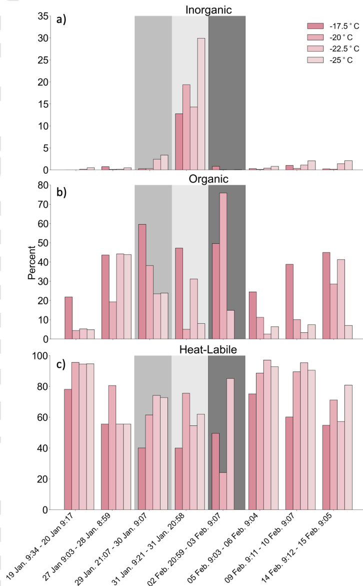
Figure 5: a) Percent of inorganic INPs, b) organic (subtraction of INPs remaining after peroxide treatment from INPs remaining after heat treatment) INPs, and c) heat-labile INPs at selected dates and temperatures. The gray shaded region represents the 3 sub-periods of the ice fog event. Times are presented in AKST.
