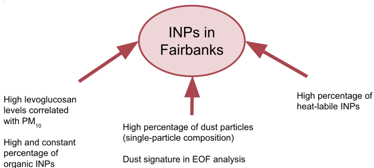
Figure 8: Schematic showing potential INP sources to be (from left to right): residential wood burning, dust, and heat-labile particles.
