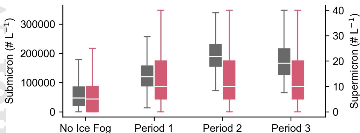
Figure 6: Boxplots of the number concentration ( \# \text{ L}^{-1} ) of submicron (0.25 – 1 \mu\text{m} , gray) and supermicron (1 – 32 \mu\text{m} , pink) aerosol particles for the three ice fog subperiods (Period 1: 29 January 9:00 – 30 January 21:00 2022, Period 2: 30 January 21:00 – 1 February 21:00 2022, and Period 3: 1 February 21:00 – 3 February 9:00 2022) and the non-fog periods. The boxes represent the 25th – 75th percentiles, with the median marked by the white lines. The whiskers represent the 5th to 95th percentiles.
