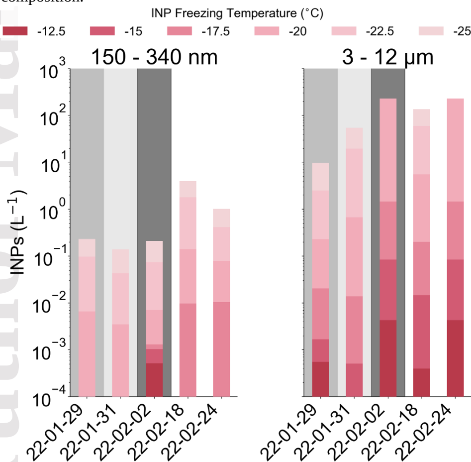
Figure 4: Cumulative INP concentrations at selected temperatures for 3 – 12 \mu\text{m} and 150 – 340 nm size bins. Gray shading indicates samples from within the ice fog period.
