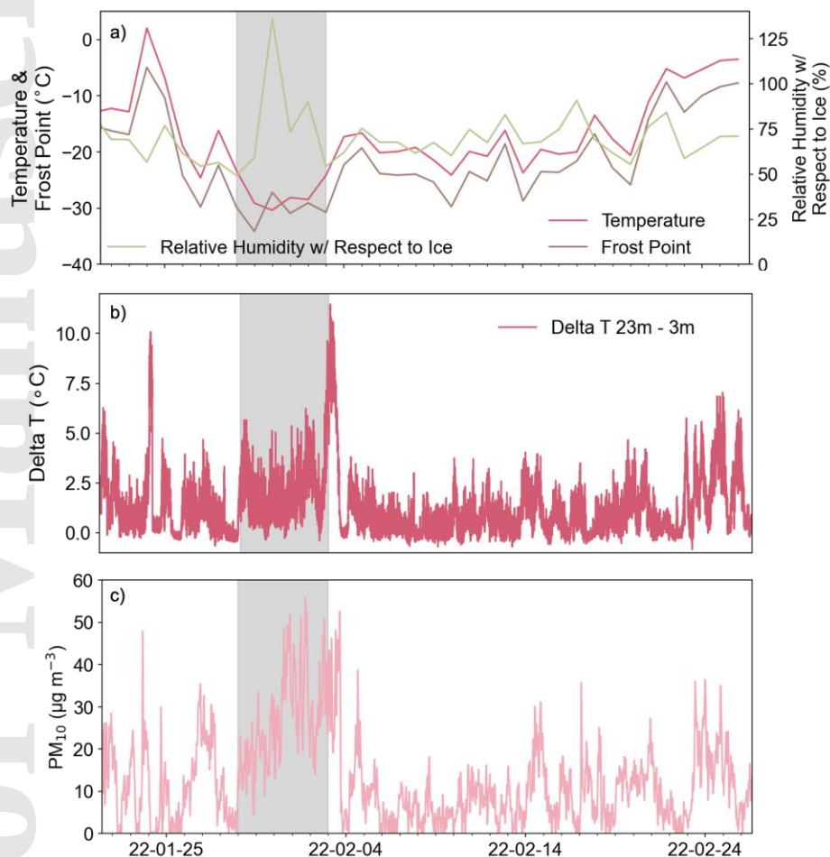
Figure 2: Time series in AKST of a) daily average meteorological parameters, including air temperature, frost point, and calculated relative humidity with respect to ice (Murphy & Koop, 2005), b) Inversion strength between 3 and 23 m, and c) PM 10 mass concentrations (30 min time resolution) from the downtown Fairbanks site during the 2022 ALPACA campaign. The gray shaded regions highlight the ice fog and pollution event during the campaign.
