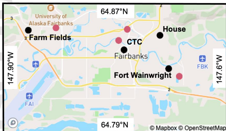
Figure 1: Map of Fairbanks, Alaska with study locations marked by black points and labeled. Power plants are marked by pink points.
