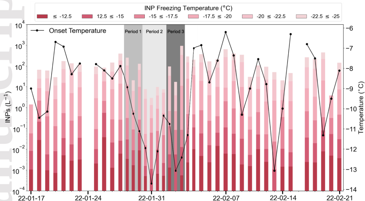
Figure 3: Cumulative INP concentrations per L of air at a representative set of freezing temperature values for each total aerosol filter sample collected in downtown Fairbanks at the CTC site. The ice fog period is shaded gray. The wider bars, collected between 17 January – 28 January and 4 February – 21 February represent the filters collected for a total of 24 hours. The narrow bars, collected between 29 January – 4 February, represent filters collected for a total of 12 hours. The first set of bars highlighted in gray represent: 1) Period 1: 29 January 9:00 – 30 January 21:00 2022, 2) Period 2: 30 January 21:00 – 1 February 21:00 2022, and 3) Period 3: 1 February 21:00 – 3 February 9:00 2022. The solid black line shows the onset freezing temperature for each filter.
