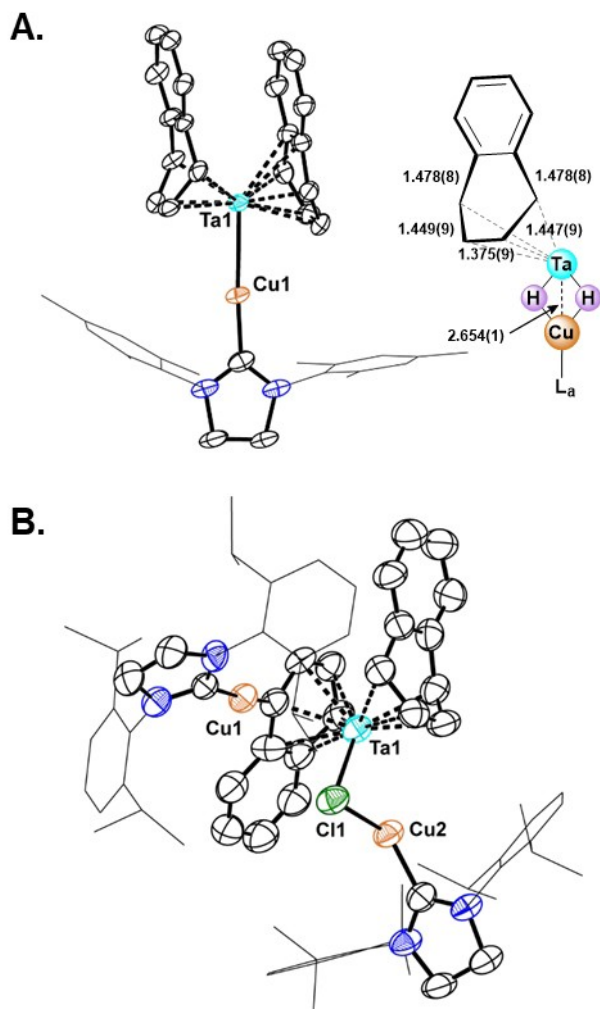
Figure 2. Single-crystal XRD structures (50% thermal anisotropic displacement ellipsoids) of 1a (A) and 2b (B). In each case, hydrogen atoms are omitted for clarity. Bond metrics (in Å) are provided for both the Ta–Cu bond and \eta^4 -naphthyl C–C bonds in 1a .
