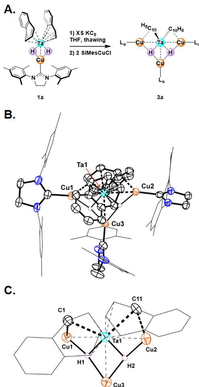
Figure 3. Synthetic pathway for mixed Cu/Ta cluster 3a (A), single crystal XRD structure of the complete TaCu 3 complex (B), and a truncated depiction (side view) of the (naph) 2 Ta-( \mu -H) 2 -Cu 3 core (C). Thermal anisotropic displacement ellipsoids are shown at the 50 % probability level and non-hydride H-atoms are omitted for clarity. The hydride H-atoms were resolved in the Fourier map and refined freely.
