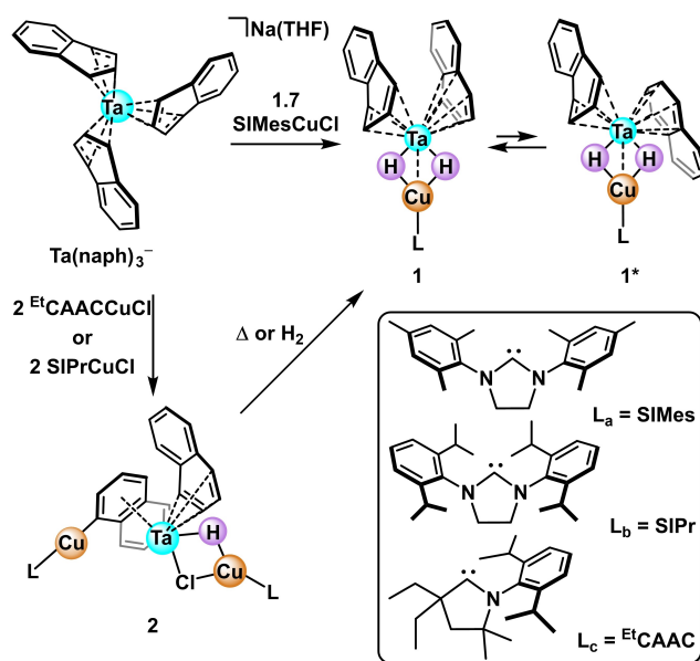
Scheme 1. Synthetic pathway to mixed Cu/Ta di- and trinuclear complexes preceding from an arene-supported metalate via metal-metal salt metathesis.
