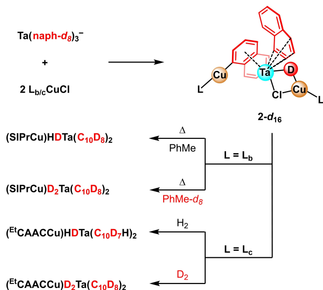
Scheme 2. Synthetic pathway to access the deuterated SIPr and ^{\text{Et}}\text{CAAC} trinuclear complexes ( 2a/b-d 16 ), and subsequent reactions to probe hydride sources in 1b and 1c .
