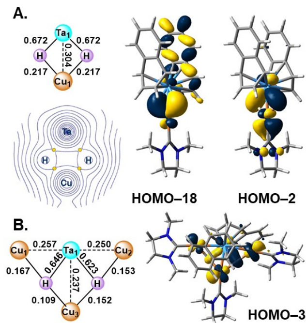
Figure 4. Select calculated Wiberg Bond Indices, QTAIM bond paths, and molecular orbitals for (\text{naph})_2\text{Ta}-(\mu\text{-H})_2\text{-Cu} (A) and (\text{naph})_2\text{Ta}-(\mu\text{-H})_2\text{-Cu}_3 (B) compounds. Isosurfaces are displayed at a 0.04 \text{eA}^{-3} level.
