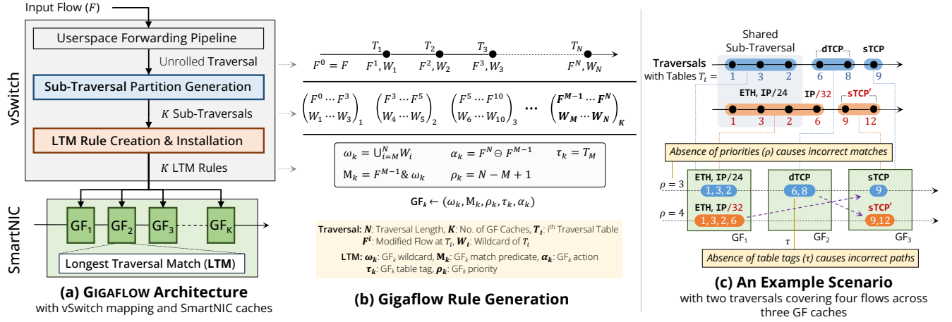
Figure 5. (a, b) High-level GIGAFLow architecture: the input flow ( F ) traverses the vSwitch userspace pipeline to produce an unrolled traversal, which is then partitioned into sub-traversals and stored as LTM rules in GIGAFLow caches. (c) Example GIGAFLow processing with two traversals partitioned across three caches, capturing four flows.
