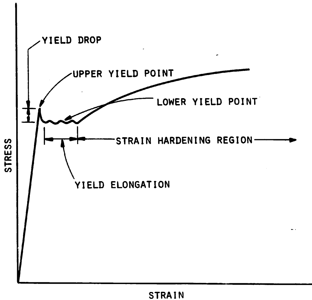
Figure 3.11 Stress-Strain Diagram for 1020-Annealed Steel (Schematic)
