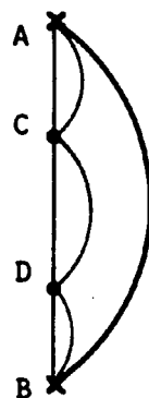
Figure 4.4 Bowing of Frank-Network Due to Applied Stress.
