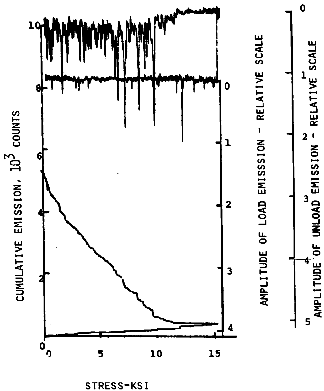
Figure 3.20 Emission from Cold-Worked High-Purity (99.99%) Aluminum.
