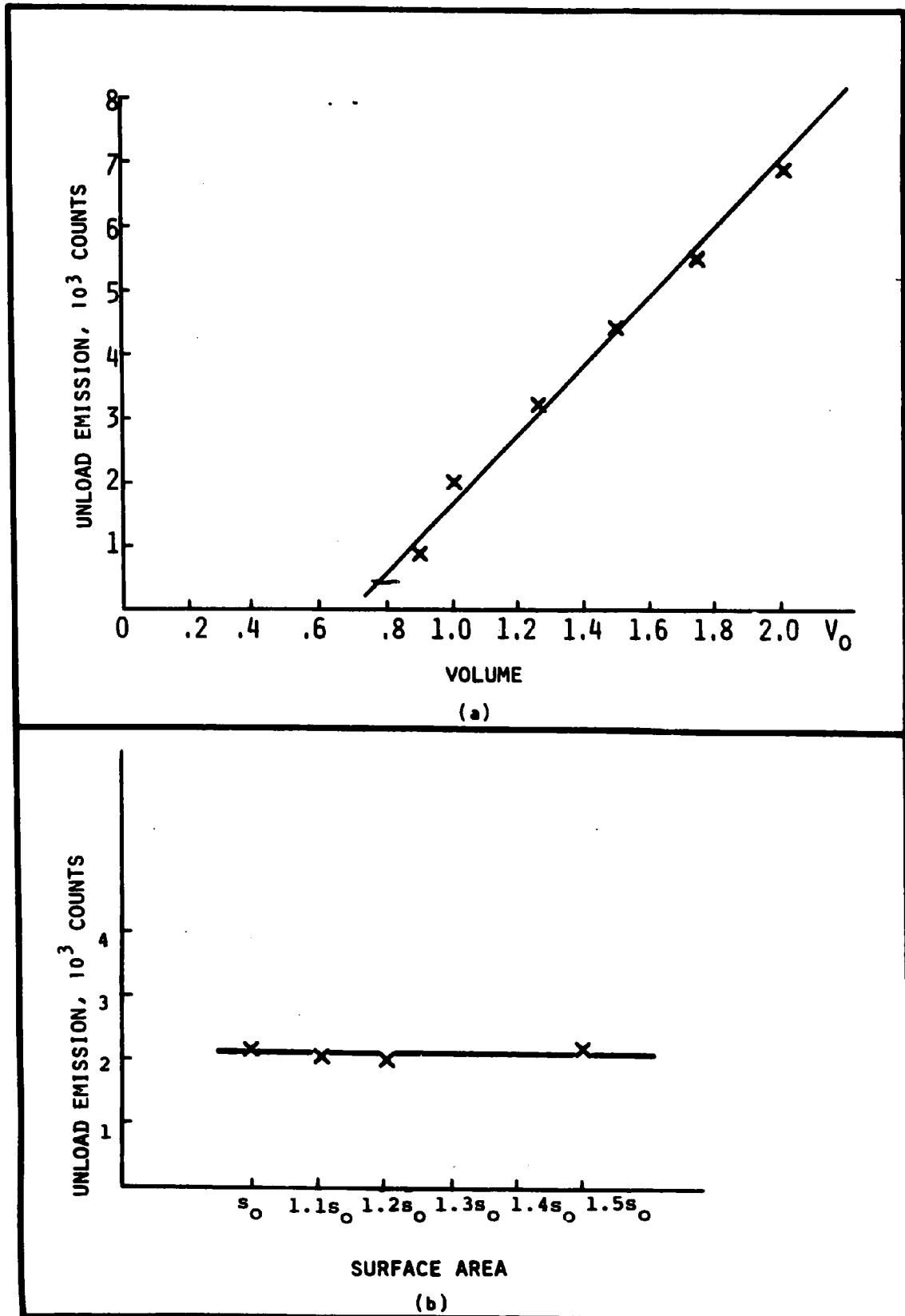
Figure 3.3 Effect of the Size of the Specimen on Unload Emission. (a) Constant Surface Area. (b) Constant Specimen Volume.
