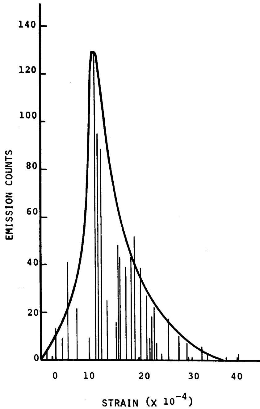
Figure 4.6 Acoustic Emission Histogram for LiF. (9)
