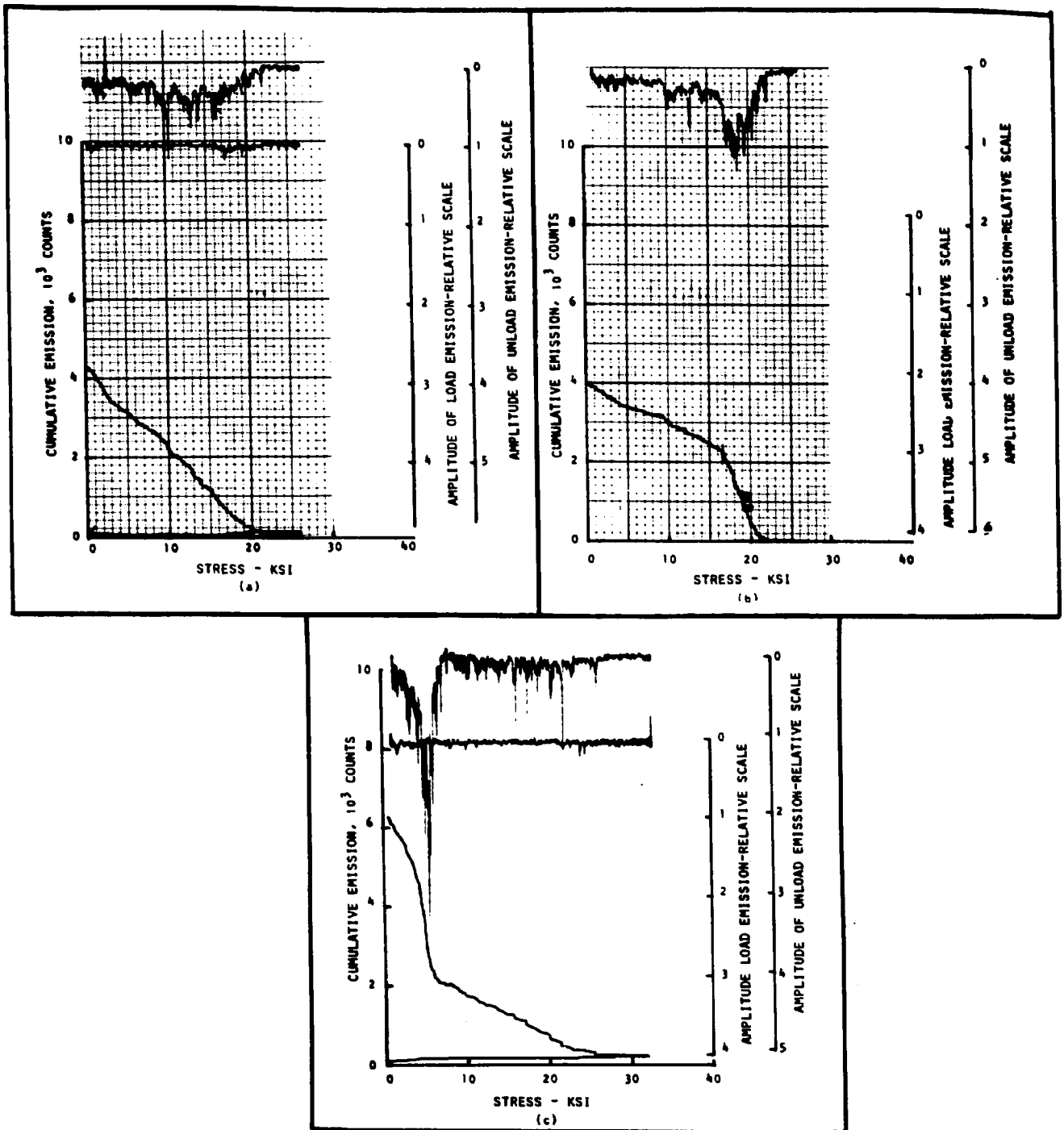
Figure 3.7 Effect of Strain-Aging on Unload Emission from 2024 Aluminum. a) Aged at Room Temperature for 116 Hours at Zero Stress, b) Aged at Room Temperature for 116 Hours at a Stress of 25 ksi, c) Aged at Room Temperature for 116 Hours After Unloading to 8 ksi.
