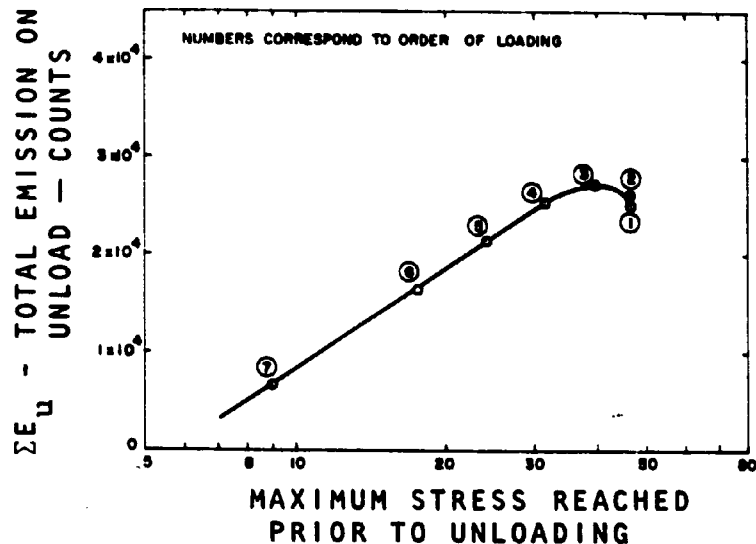
Figure 1.4 Dependence of the Unload Emission on the Maximum Stress Reached Prior to Unloading the Specimen.
