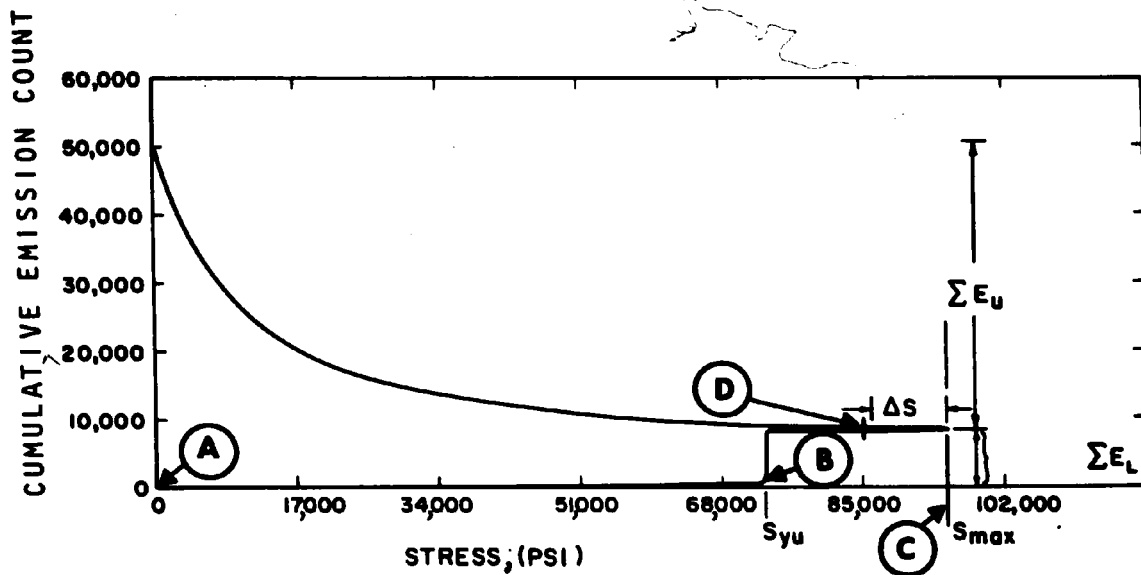
Figure 1.2 Dependence of the Cumulative Acoustic Emission in Steel on an Axial Tensile Stress. (8)
