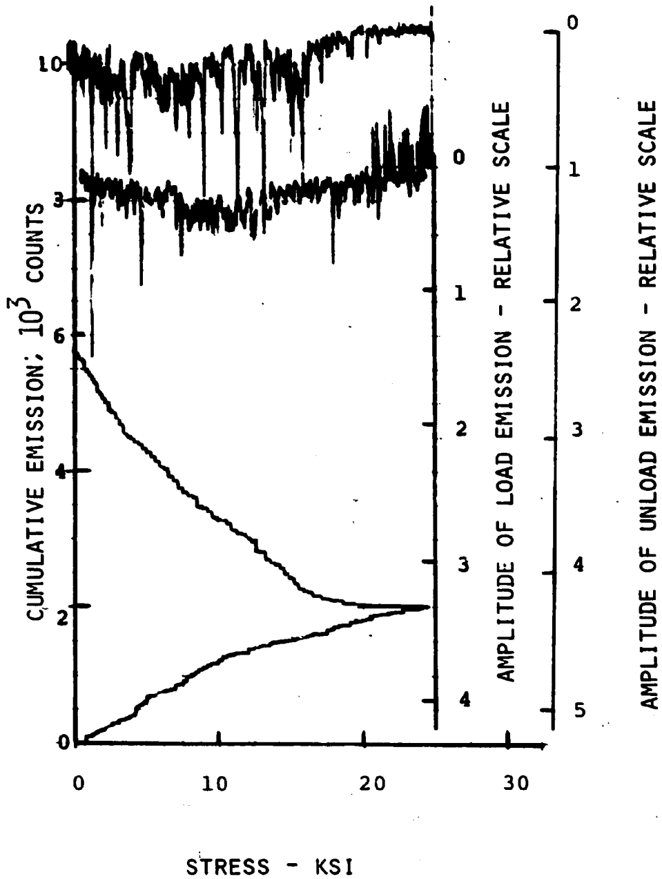
Figure 3.17 Emission from Overaged 2024 Aluminum. (Aged at 600°F for 100 Hours after Solution-Treating at 975°F for Four Hours).
