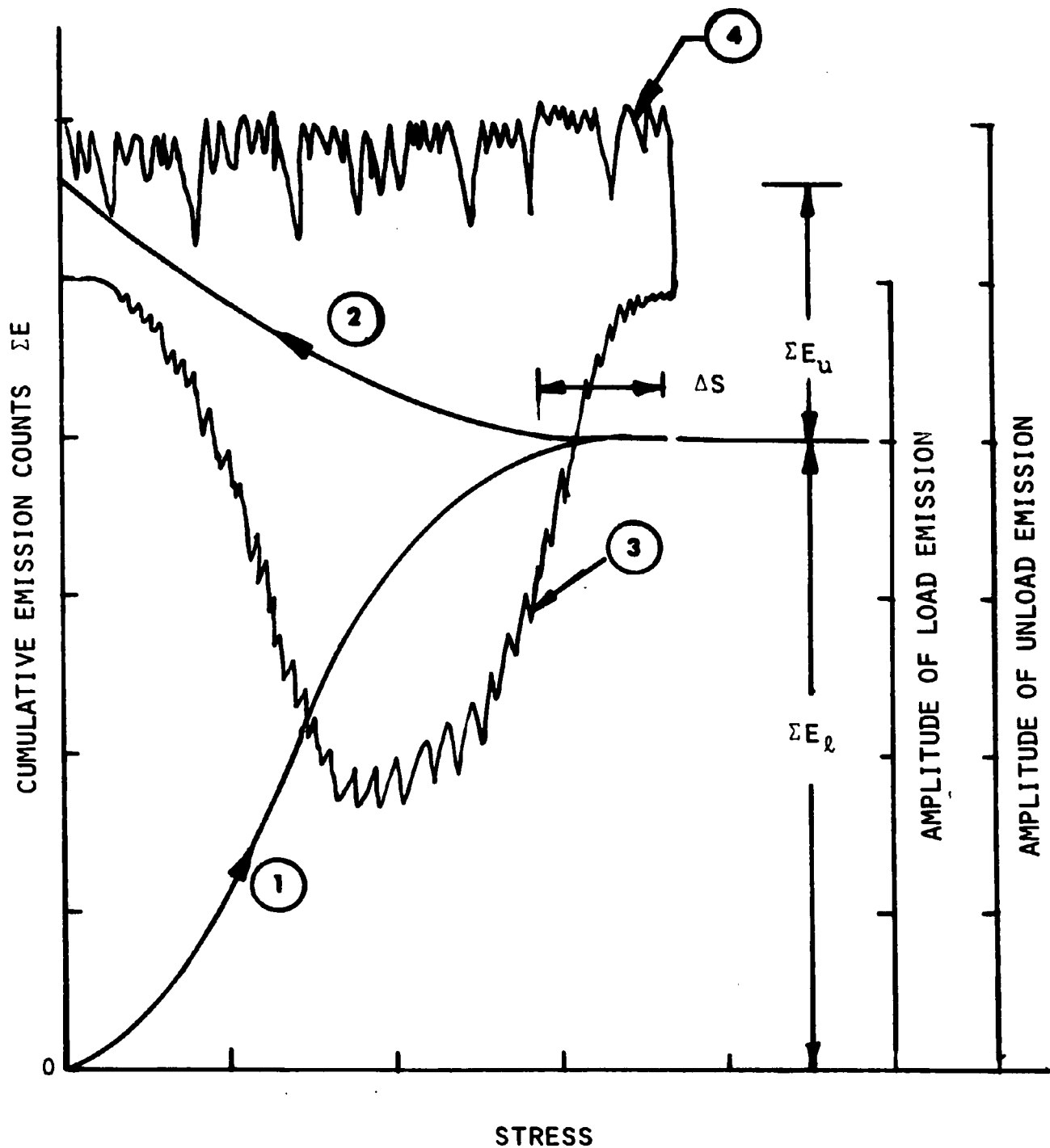
Figure 4.2 Emission Spectra (Schematic).
