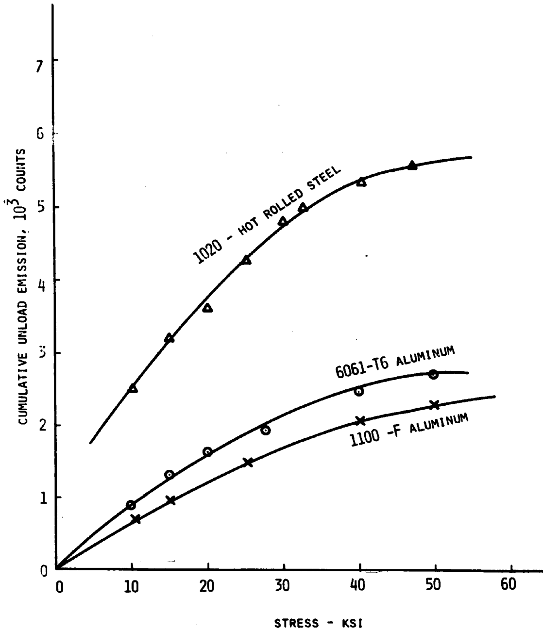
Figure 3.6 Cumulative Unload Emission Count, versus Maximum Applied Stress.
