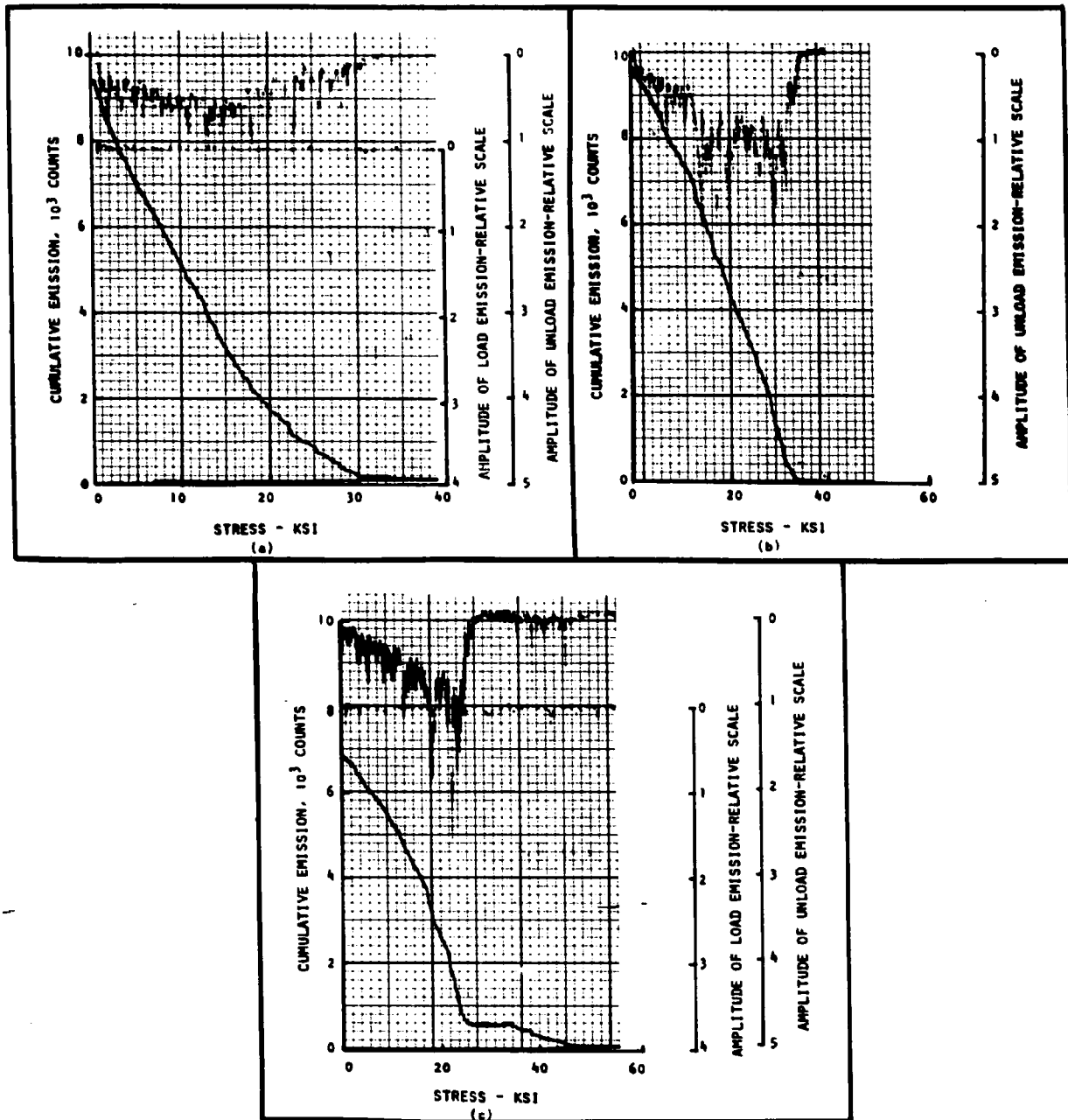
Figure 3.8 Effect of Strain-Aging on Unload Emission from 1020 Steel. a) Aged for 20 Hours at 180°F at Zero Stress, b) Aged at 180°F for 20 Hours at a Stress of 40 ksi, c) Aged at 180°F for 20 Hours After Unloading to 30 ksi.
