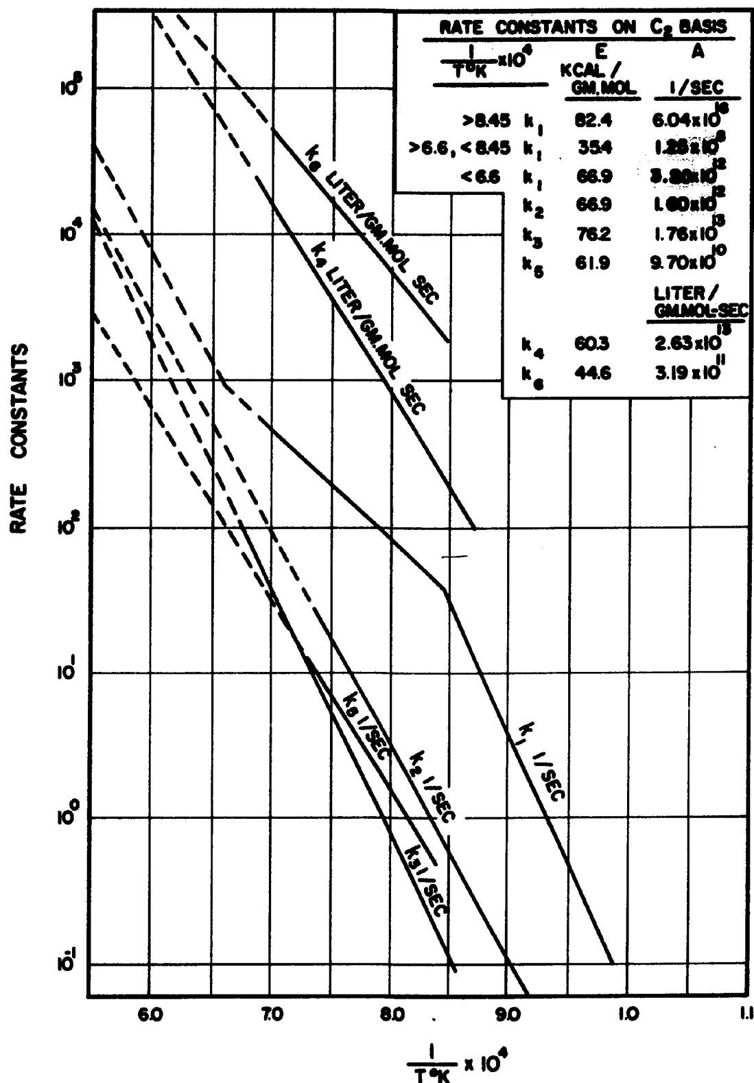
Figure 36. Rate Constants for the Six Major Reactions.
