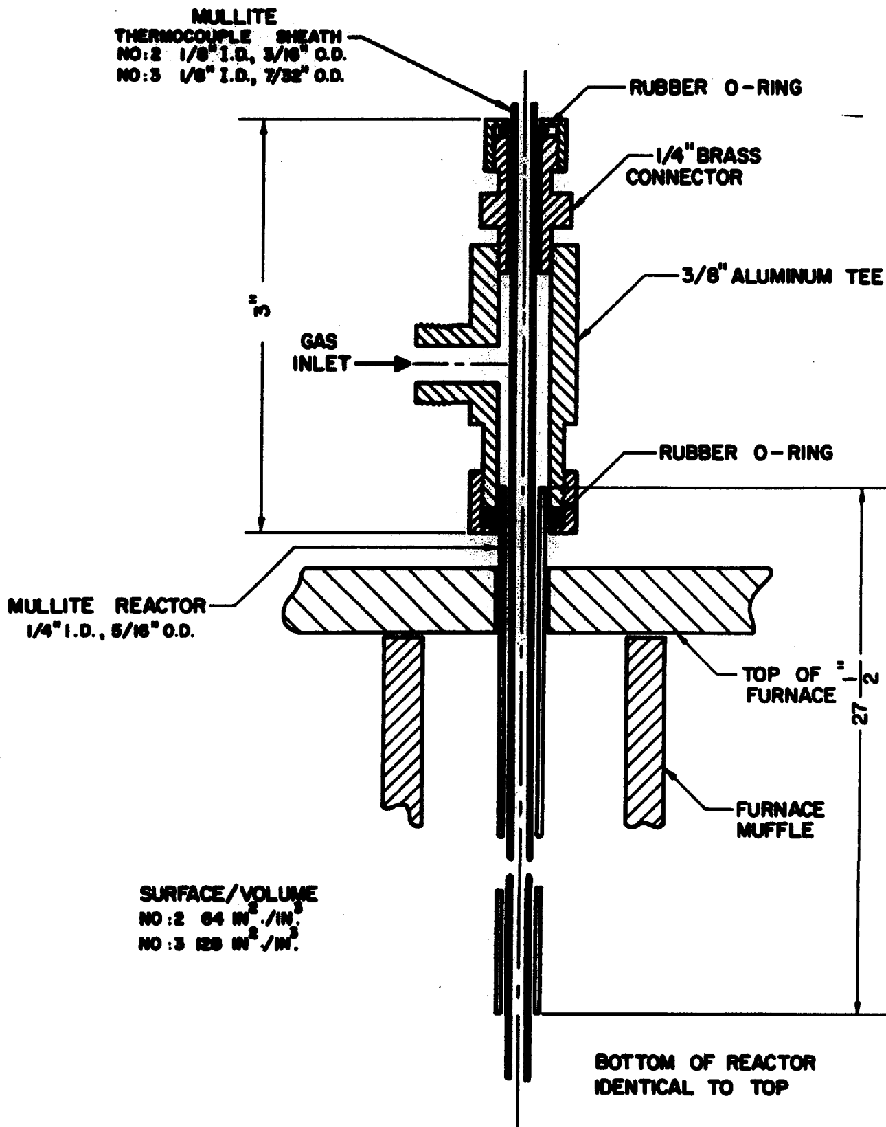
Figure 8. Constructional Details of the Annular Reactors (Nos. 2 and 3).
