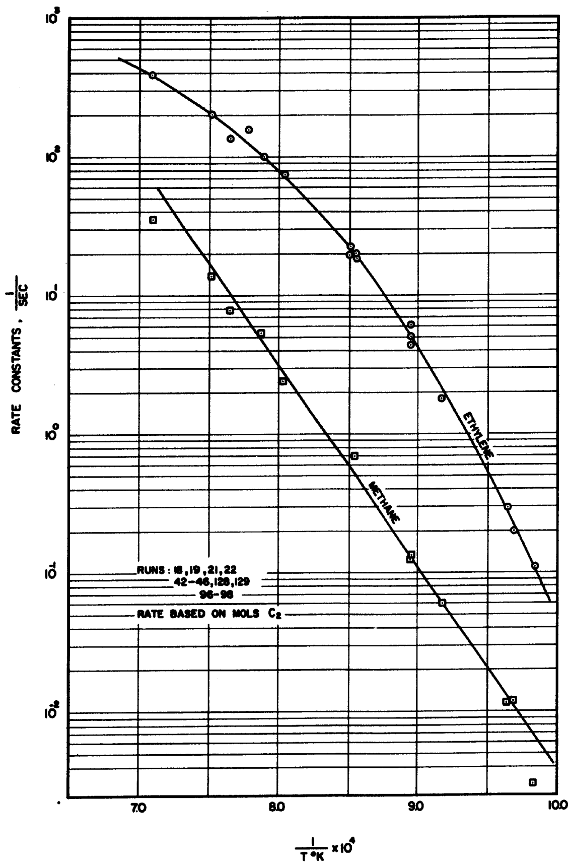
Figure 15. First Order Rate Constants for Formation of Ethylene and Methane from Ethane.
