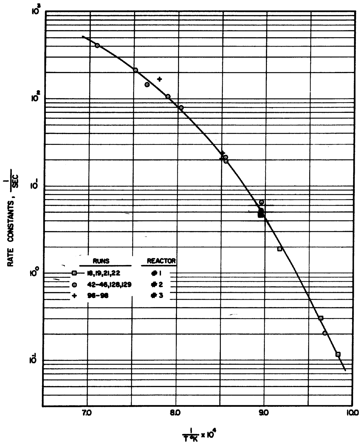
Figure 13. First Order Rate Constants for the Disappearance of Ethane.
