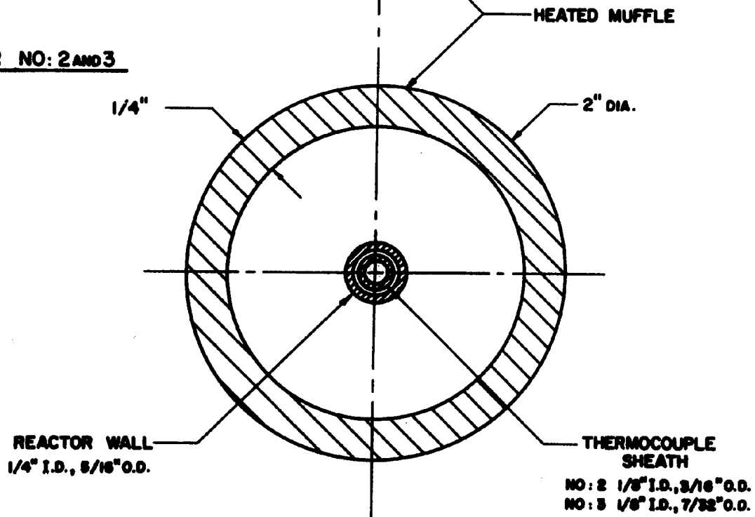
Figure 17. Radial Section Through Reactors Showing Location of Thermocouples.
