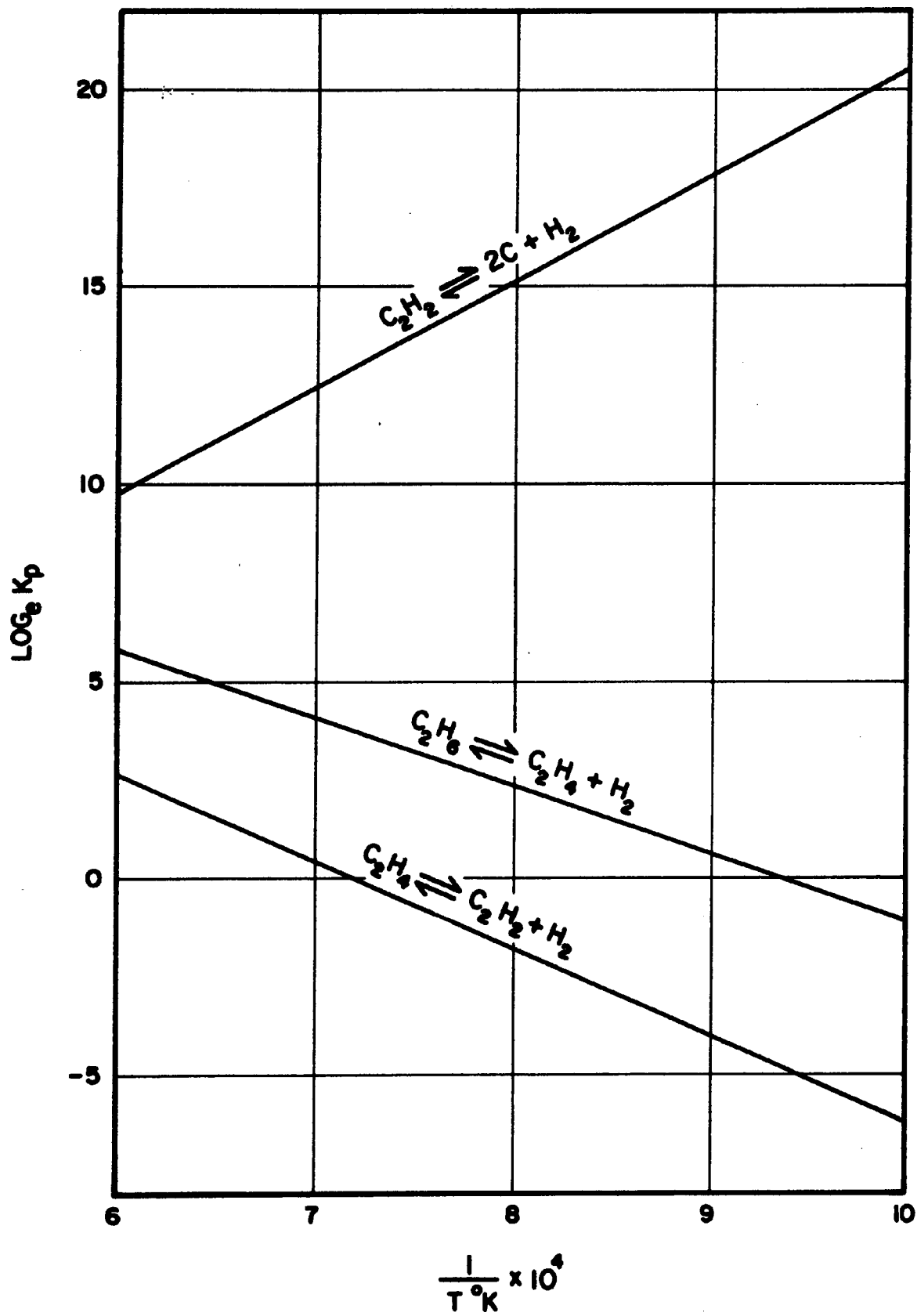
Figure 1. Equilibrium Constants in Atm. (Free Energy Data Ref. (2)).
