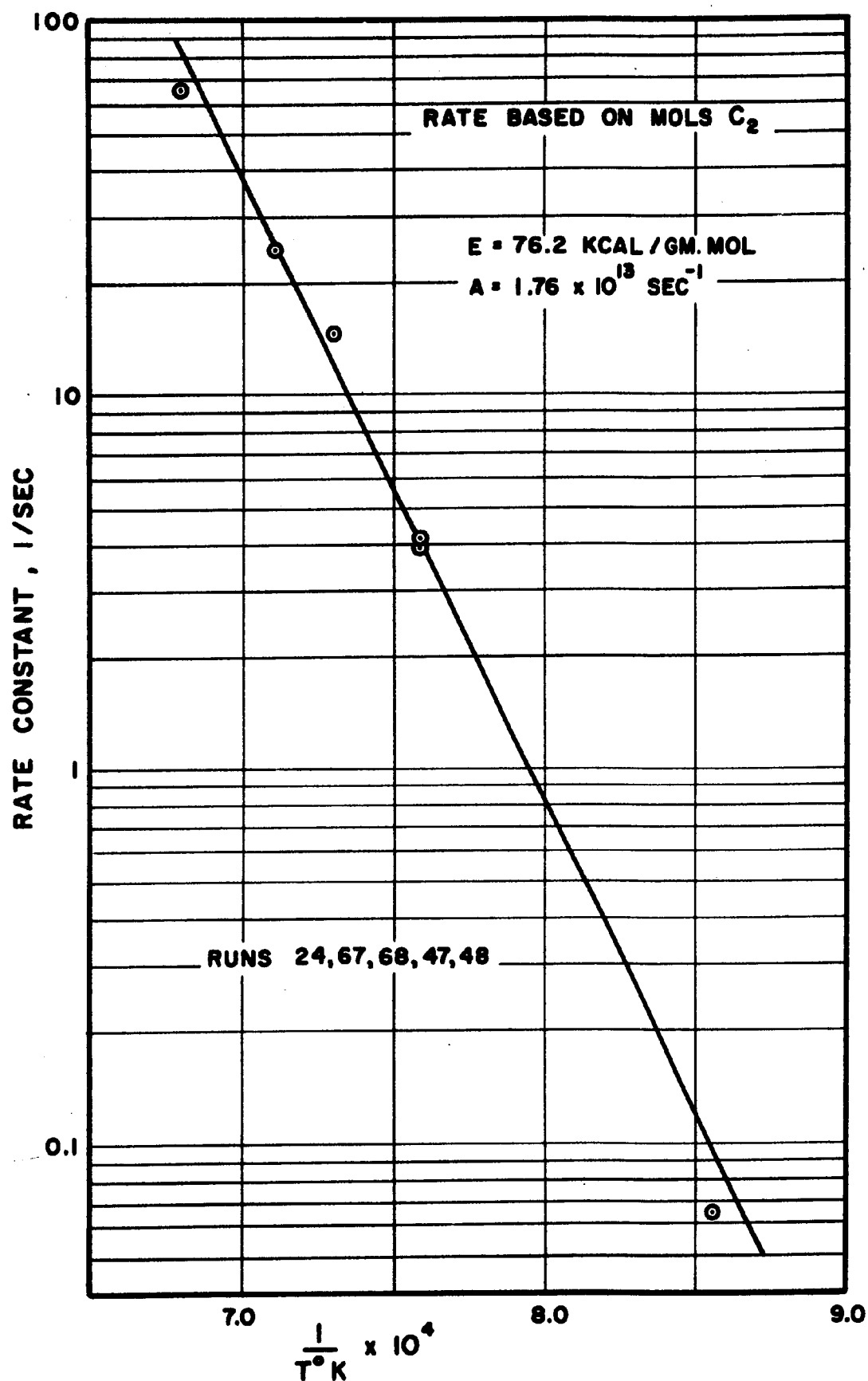
Figure 22. Acetylene Formation from Ethylene First Order Rate Constants.
