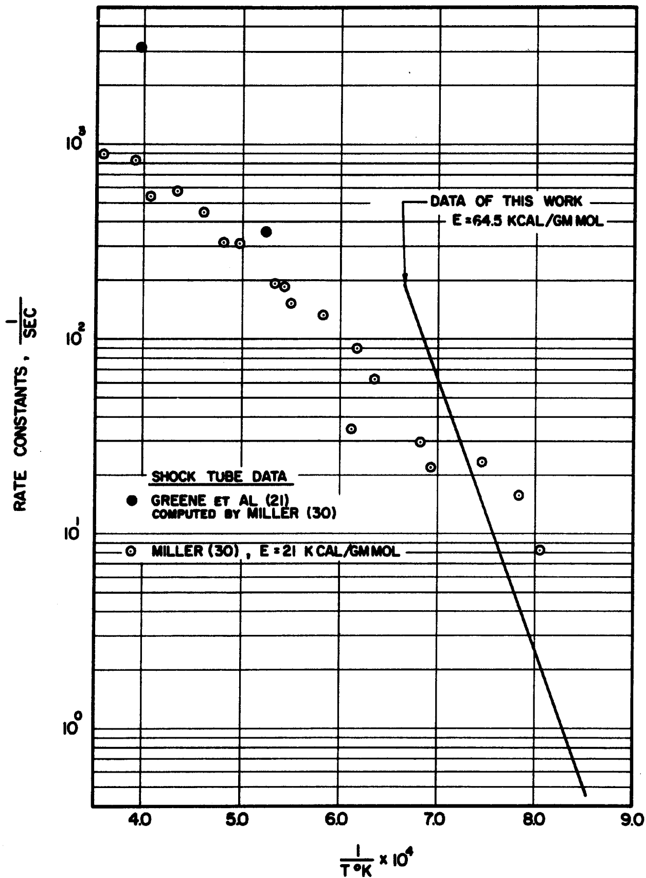
Figure 24. Ethylene Disappearance First Order Rate Constants, a Comparison with Literature Data.
