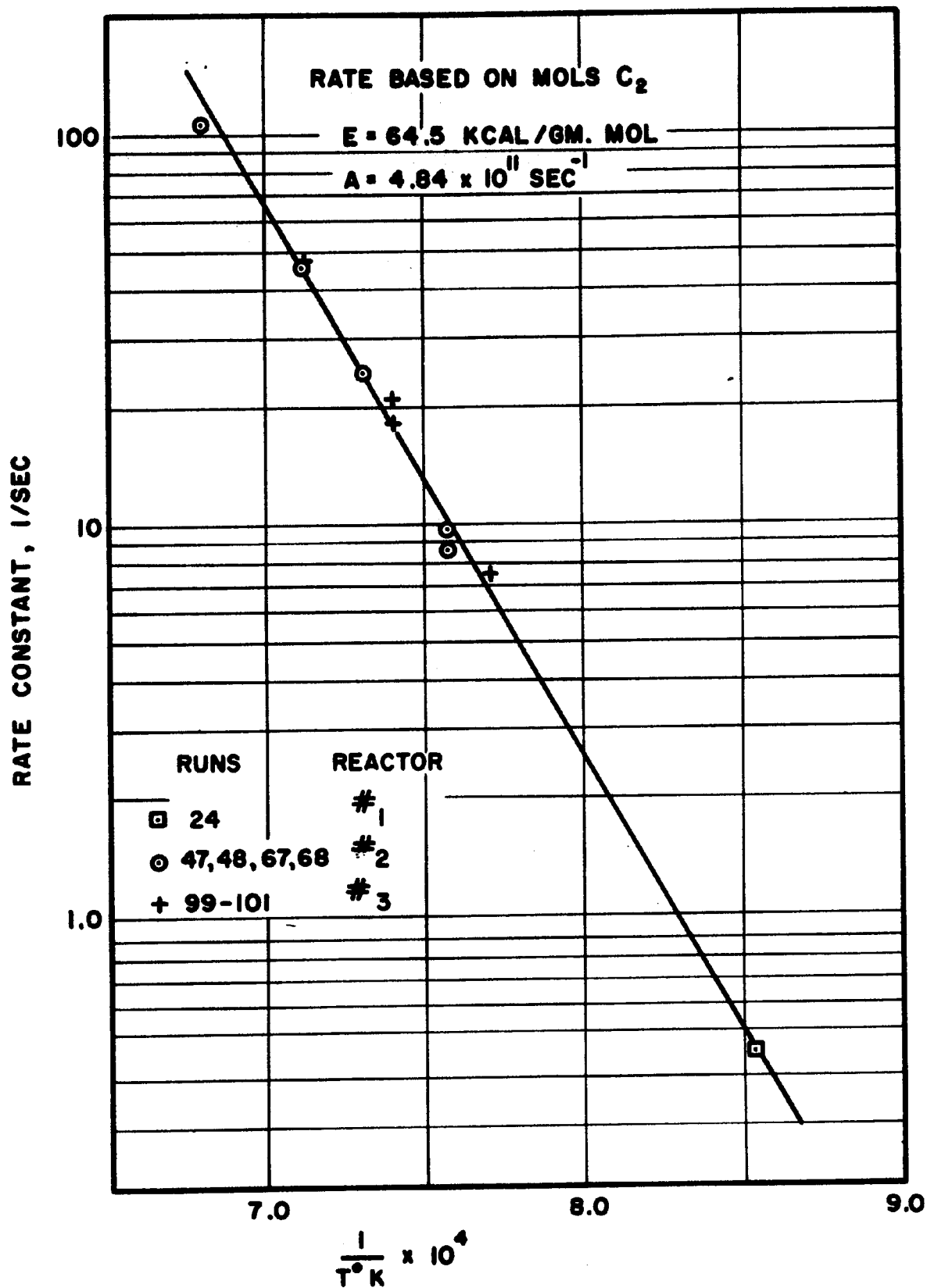
Figure 21. Ethylene Disappearance First Order Rate Constants.
