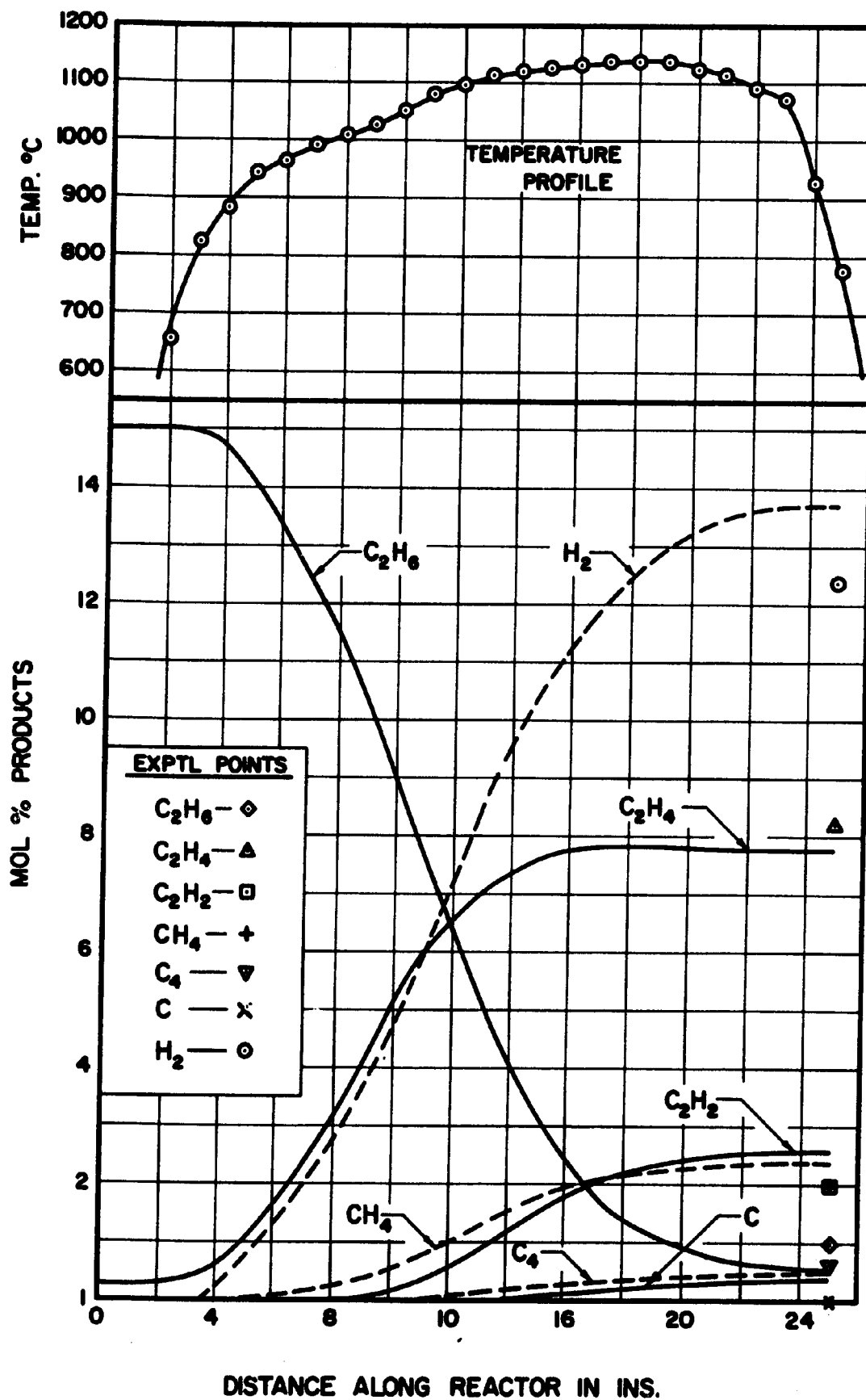
Figure 38. Calculated Product Distribution Throughout the Reactor for Run 129.
