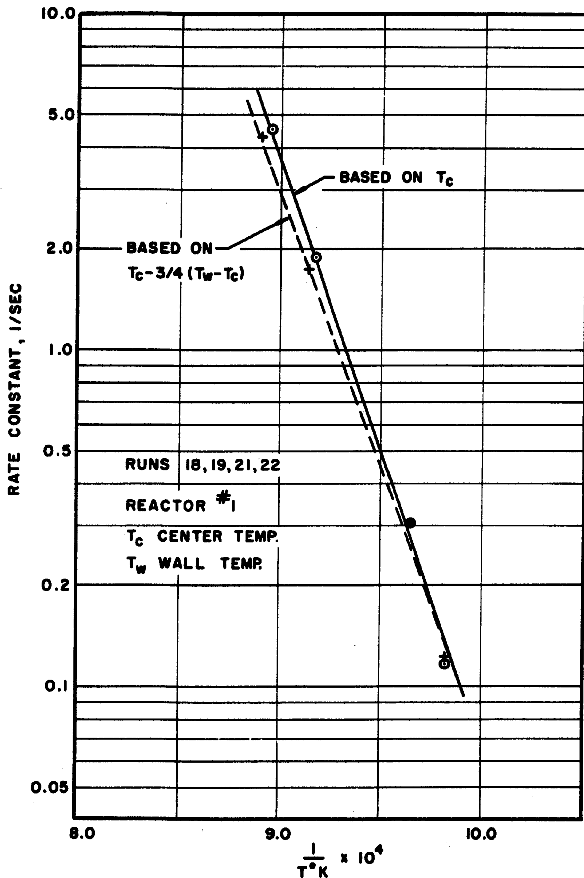
Figure 18. Effect of Radial Temperature Distribution.
