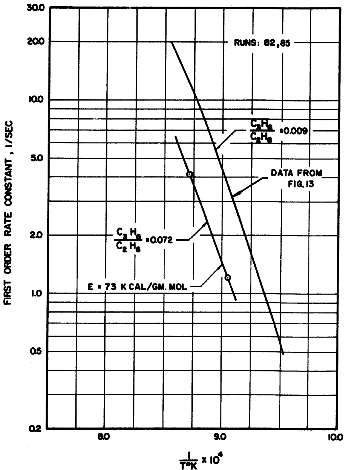
Figure 35. Ethane Decomposition Activation Energy for Reaction Inhibited with Propylene.
