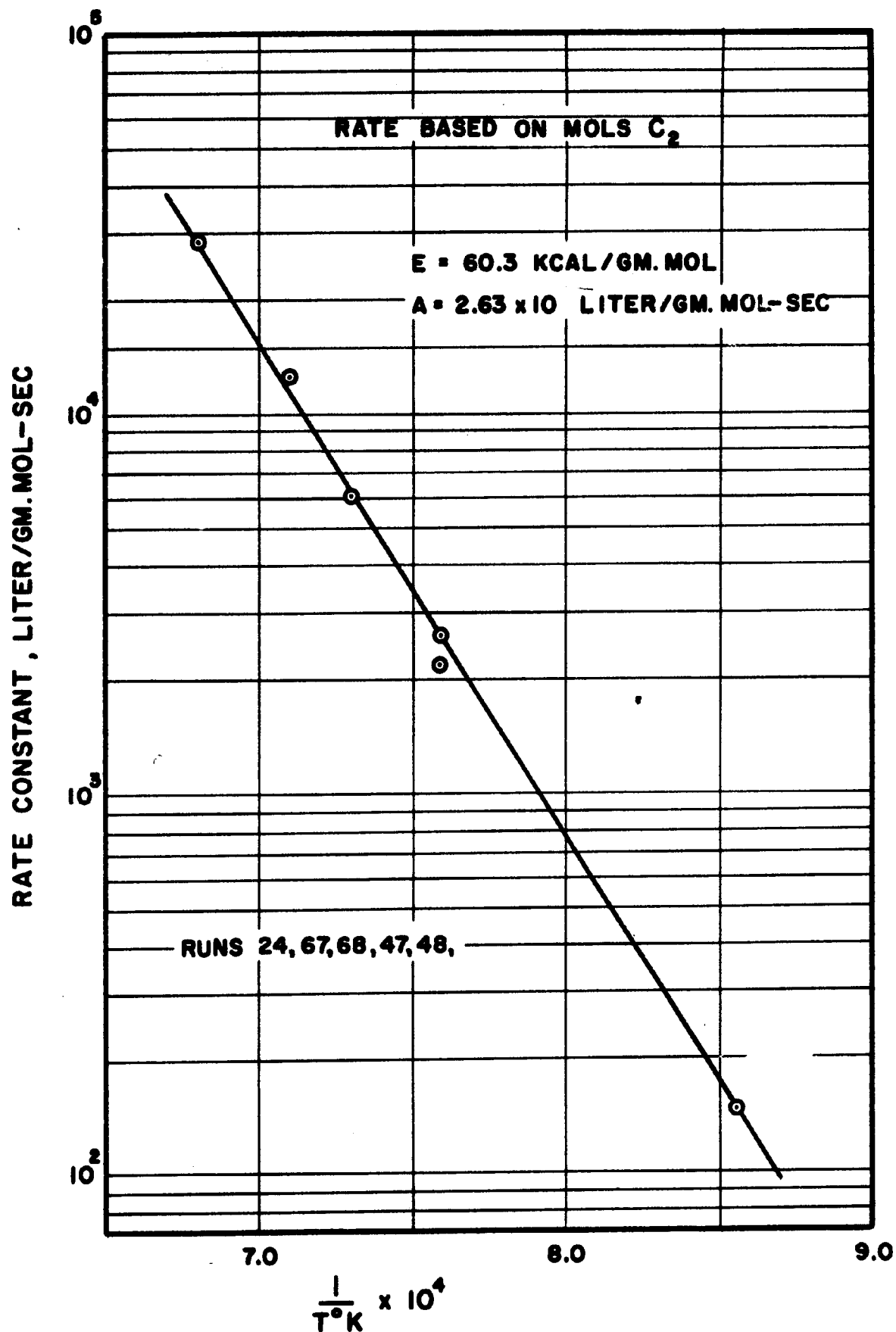
Figure 23. Polymerization of Ethylene Second Order Rate Constants.
