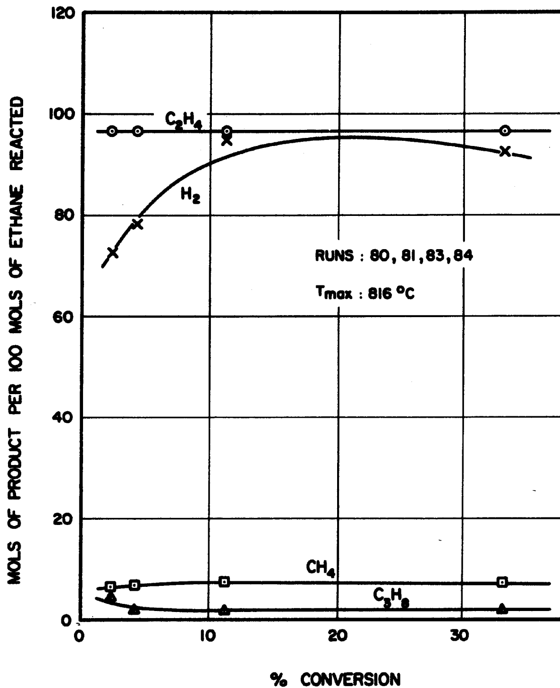
Figure 10. Product Distribution in Ethane Decomposition.
