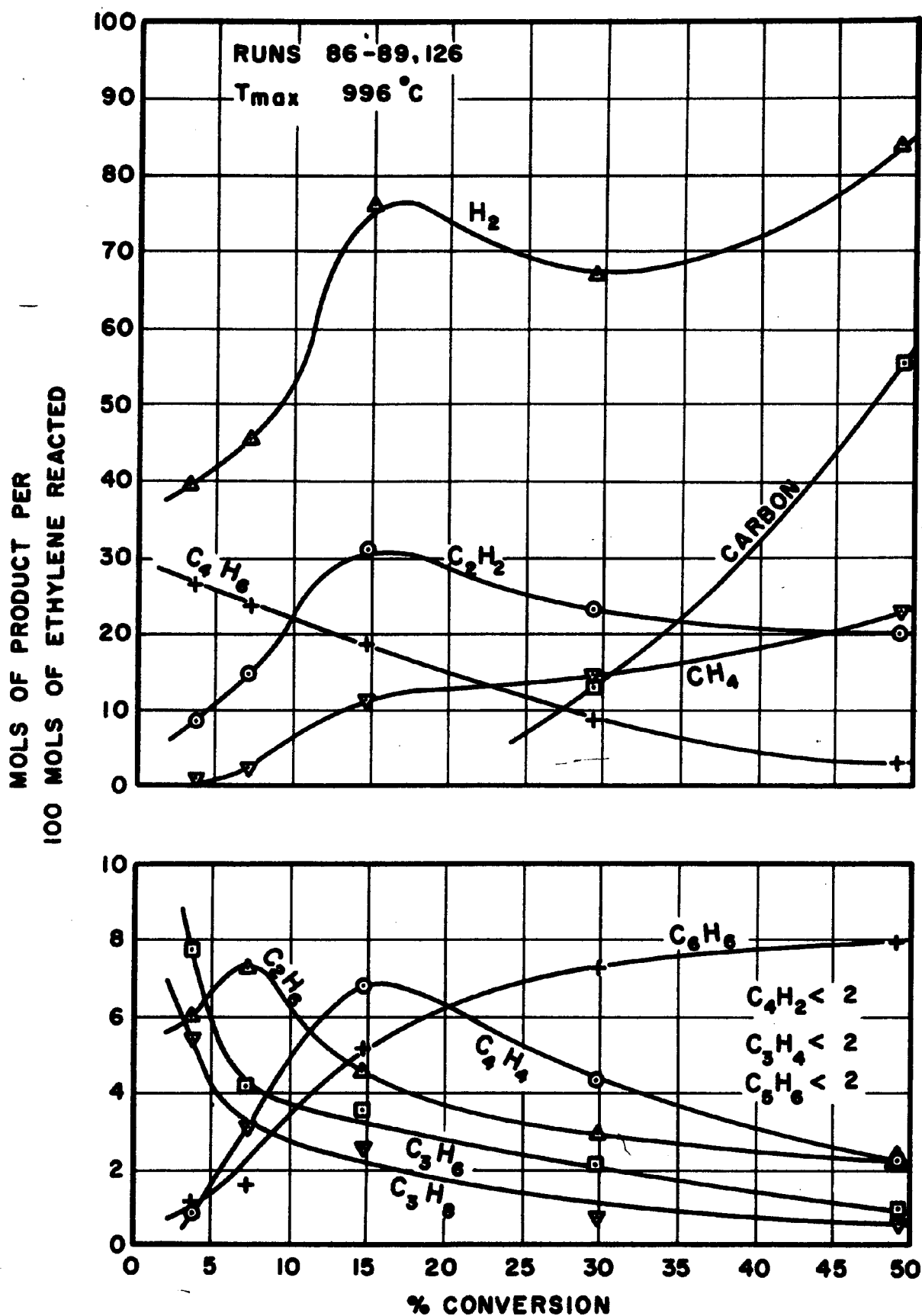
Figure 19. Product Distribution in Ethylene Decomposition.
