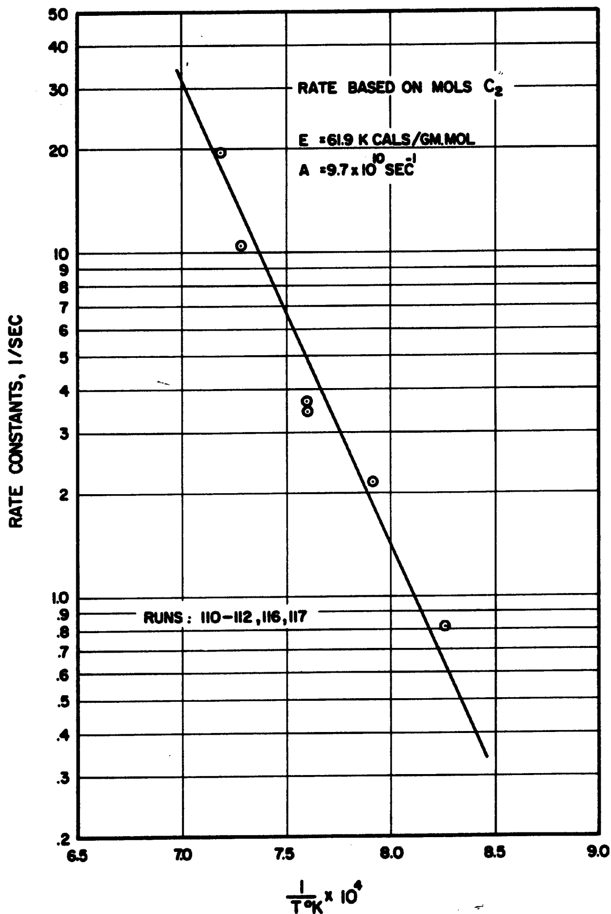
Figure 28. Carbon Formation from Acetylene First Order Rate Constants.
