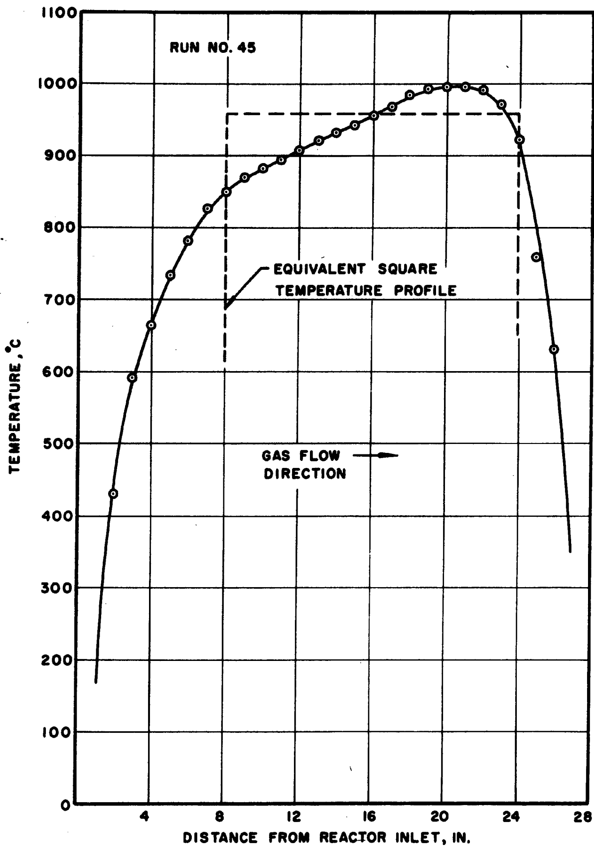
Figure 12. Typical Experimental Temperature Profile.
