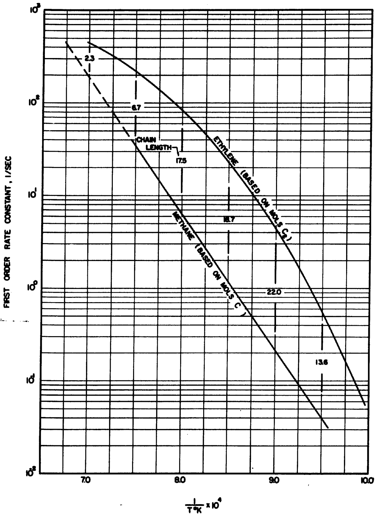
Figure 34. Chain Lengths for Ethane Decomposition.
