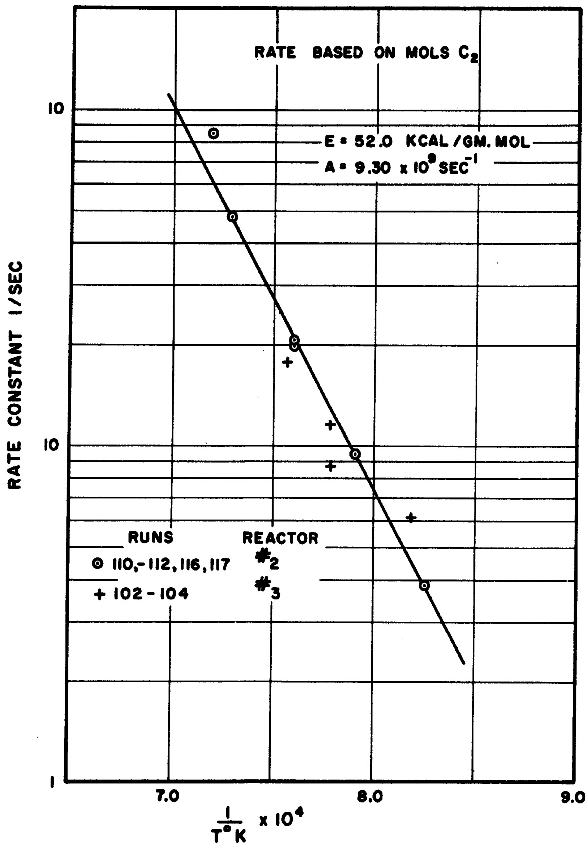
Figure 27. Acetylene Disappearance First Order Rate Constants.
