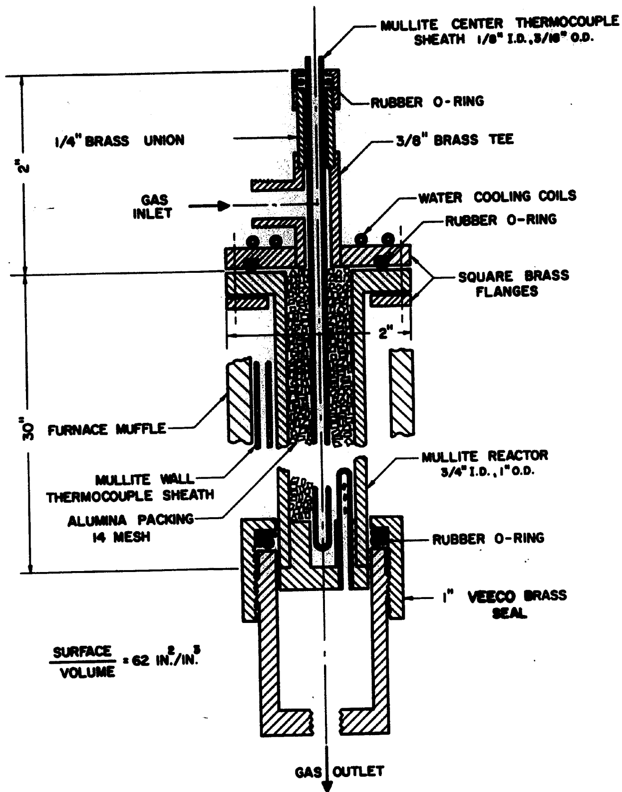
Figure 7. Constructional Details of the Packed Reactor (No. 1).
