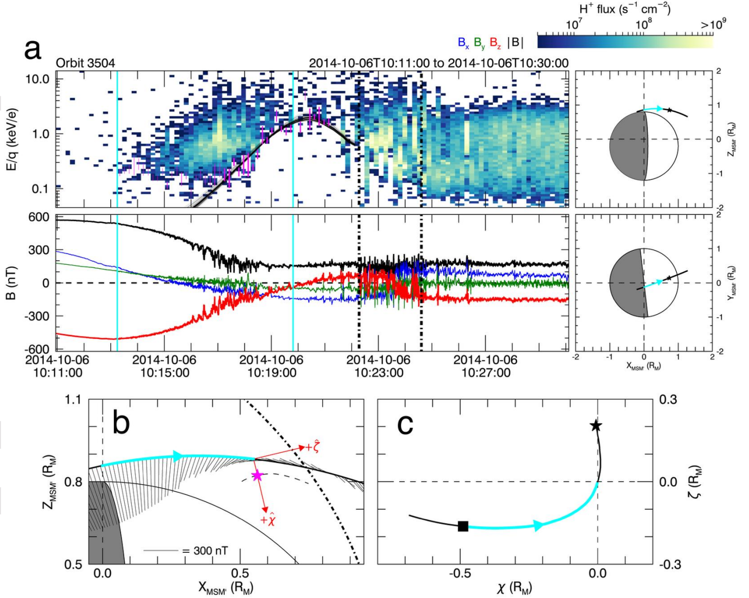
Figure 7. (a) MESSENGER dayside observations in the same format as Figure 5. The two dash-dotted lines mark the magnetopause boundary layer. (b) Spacecraft trajectory in X - Z_{MSM'} coordinates similar to Figure 2a. The magenta star marks the projected \chi_0 location at \zeta = 0 and the curved dashed line traces the field line geometry inferred from observations at the spacecraft. (c) Spacecraft trajectory in \chi - \zeta coordinates similar to Figure 2c, where the black square marks the terminator crossing and the black star the planetmost magnetopause crossing.
