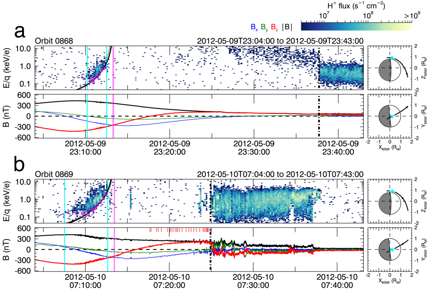
Figure 5. MESSENGER observations from two sequential orbits covering the same portion of the spacecraft's trajectory (i.e., features can be compared directly between the plots). These orbit observations are in the same general format as in Figure 1 with the addition of dispersion fit features. Similar to Figure 4c, a random subsample of fits is shown as transparent black lines, magenta bars mark \bar{E}_{\min} \pm \delta \bar{E}_{\min} and are scaled by their relative use in the fits, and the vertical magenta line marks the extrapolated crossing of the open-closed boundary. The red ticks in (b) mark flux transfer events. Proton fluxes are in differential energy flux units.
