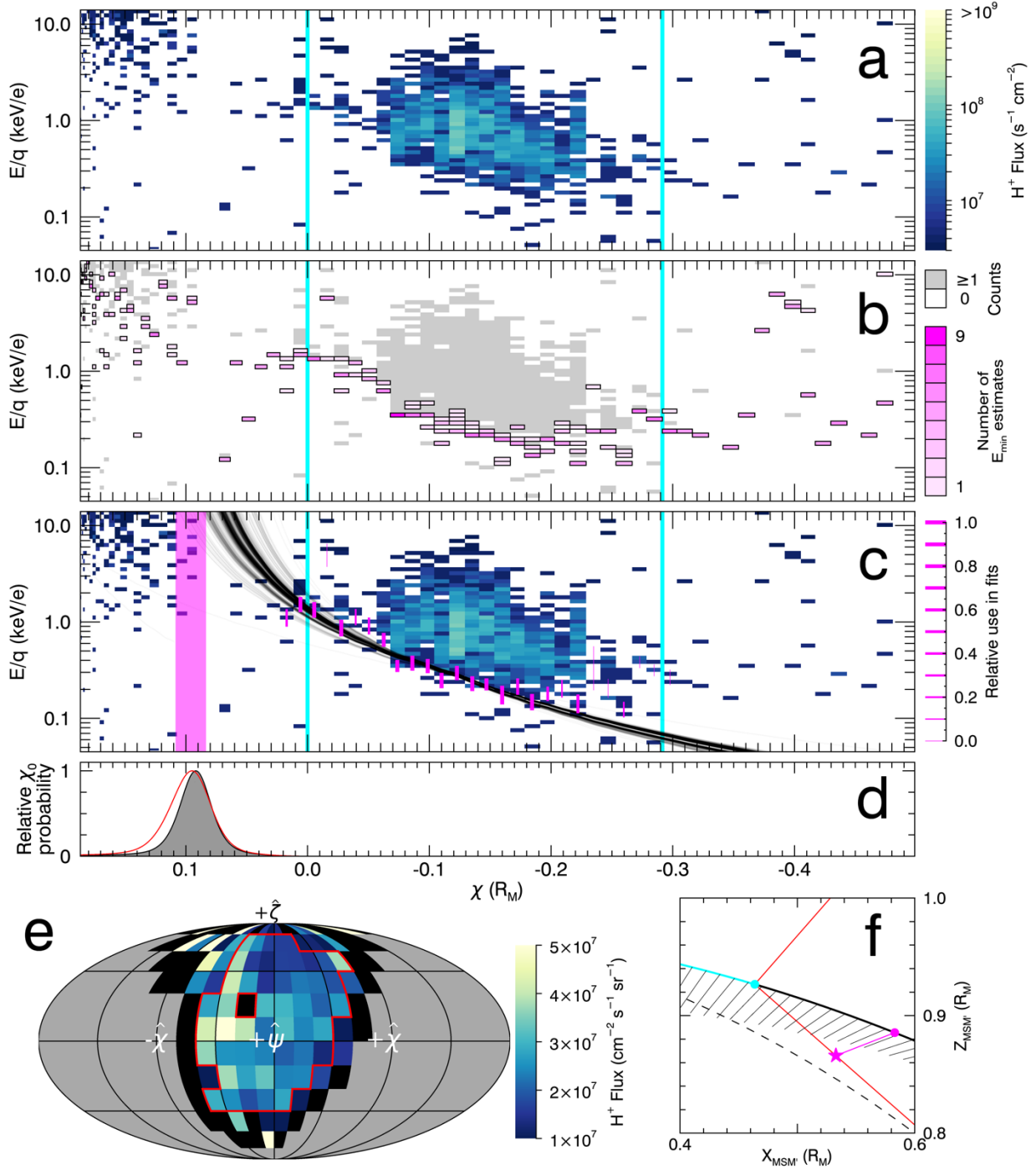
Figure 4. Illustration of determining \bar{E}_{\min} and fitting the dispersion for the cusp crossing in orbit 1915. (a) Proton differential flux in the field-aligned coordinate frame. The Raines et al. (2022) cusp boundaries are marked in cyan. (b) The number of E_{\min} estimates overlaid on the proton distribution where white indicates zero counts and grey indicates non-zero counts. (c) Vertical magenta bars mark \bar{E}_{\min} \pm \delta \bar{E}_{\min} for scans used in dispersion fitting where the thickness indicates how frequently it was used in individual fits (transparent black traces). The shaded magenta region marks \chi_0 extrapolated to MESSENGER's orbit. (d) Probability density
