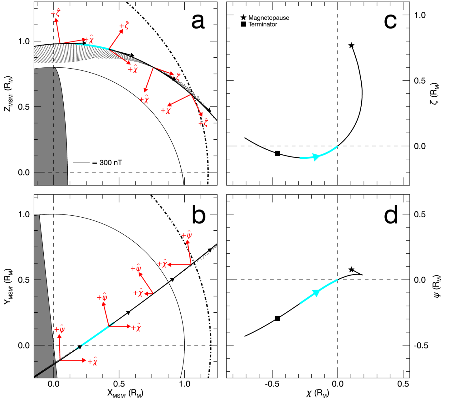
Figure 2. MESSENGER's trajectory through the dayside magnetosphere during orbit 1915 (2013-04-24T00:20 to 00:55). (a) X - Z_{\text{MSM}'} projection and (b) X - Y_{\text{MSM}'} projection. The cusp crossing from Raines et al. (2022) is highlighted in cyan. The thin lines indicate the direction of the average magnetic field during each FIPS scan and the dash-dotted line marks a fitted magnetopause ( Winslow et al., 2013 ). The red arrows indicate directions of the field-aligned frame at various points in the interval, and the black arrows indicate the direction of spacecraft's motion at those points. (c) \chi - \zeta projection and (d) \chi - \psi projection where the square marks the terminator crossing, the star the magnetopause crossing, and the arrow the spacecraft's direction of travel.
