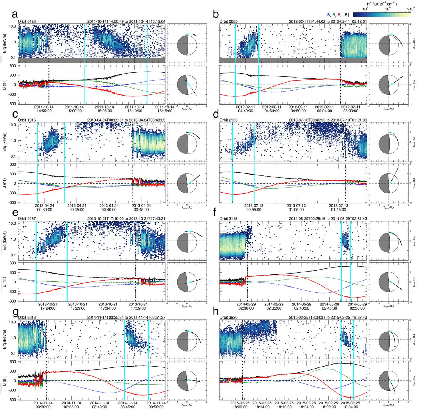
Figure 1. Examples of coherent, large-scale “classical” energy-latitude dispersions in Mercury’s northern magnetospheric cusp (cyan). For each dayside magnetosphere crossing: (top left) FIPS proton differential energy flux where white indicates no counts and dark grey are energies outside of the instrument’s E/q range; (bottom left) magnetic field; and trajectory projected onto the (top right) X-Z_{MSM} and (bottom right) X-Y_{MSM} planes. The planetward edge of the magnetopause is indicated by the dash-dotted line and by the black star.
