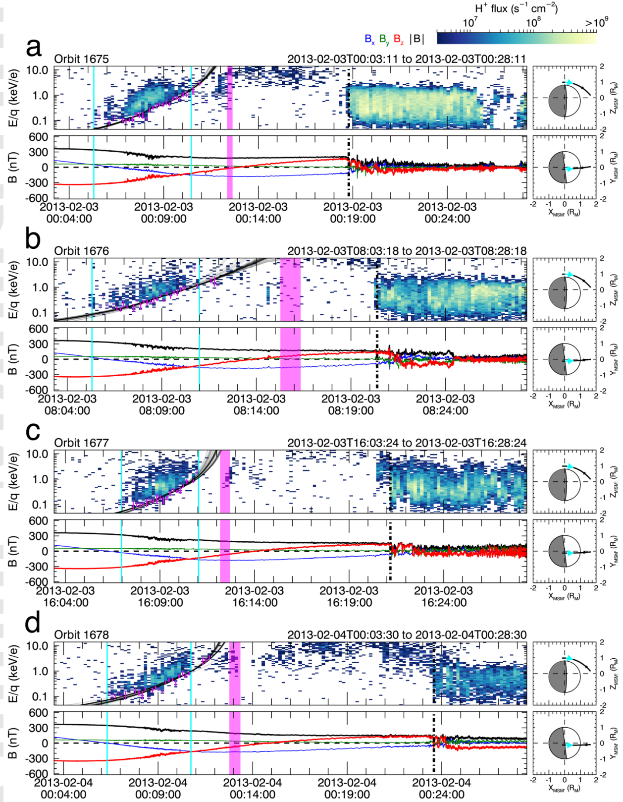
Figure 6. Four sequential orbits in the same format as Figure 5.
