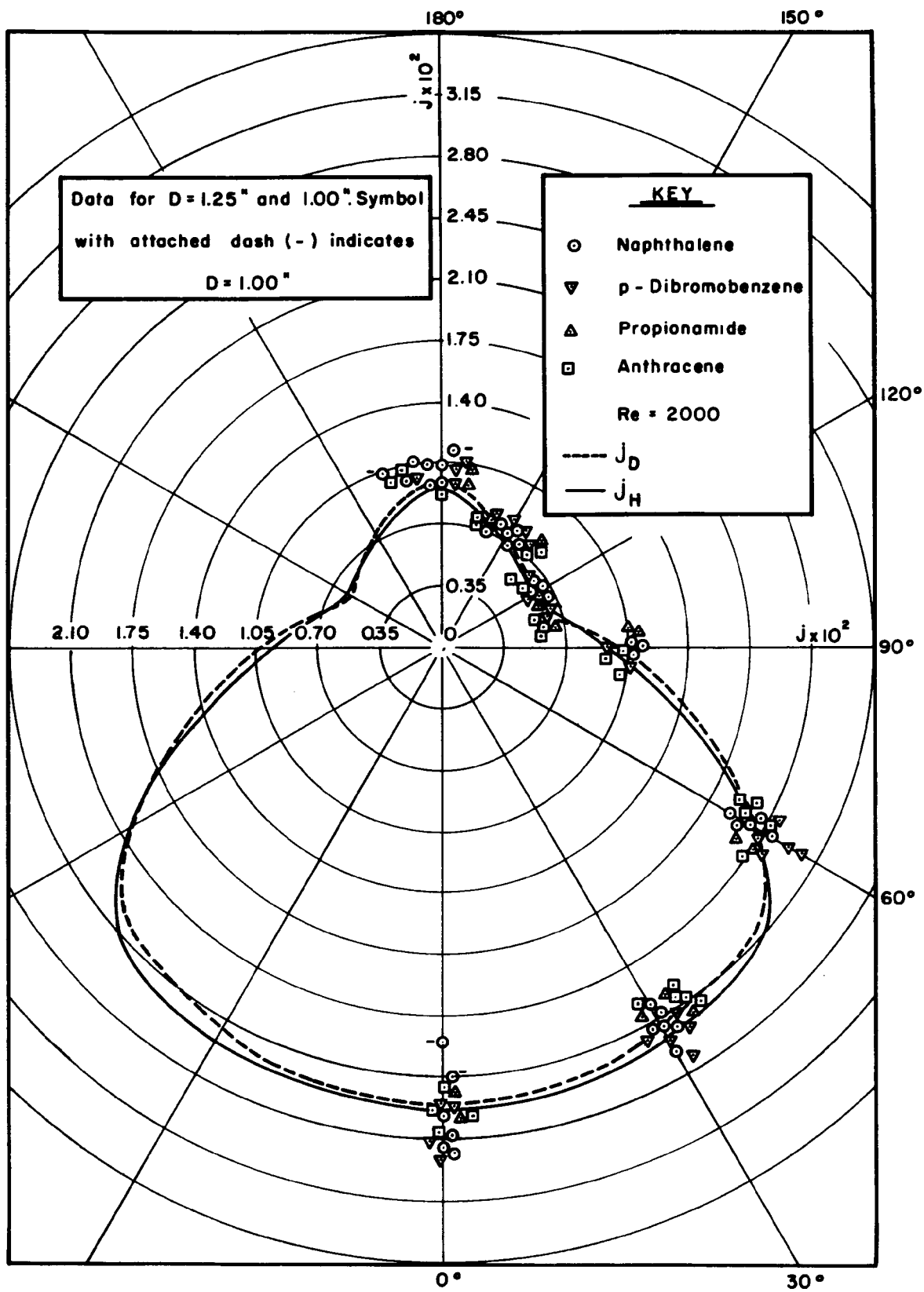
Figure 6c. Polar Diagrams for Heat and Mass-Transfer j -Factor Distributions at Re = 2000 . Data for \theta = 0^\circ, 30^\circ, 60^\circ, 90^\circ, 120^\circ, 150^\circ , and 180^\circ .
