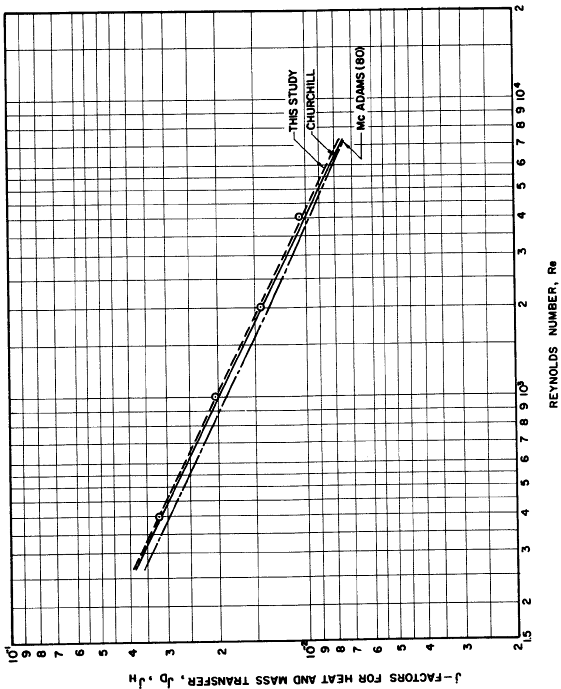
Figure 9. Correlation of Average Mass-Transfer Data.
