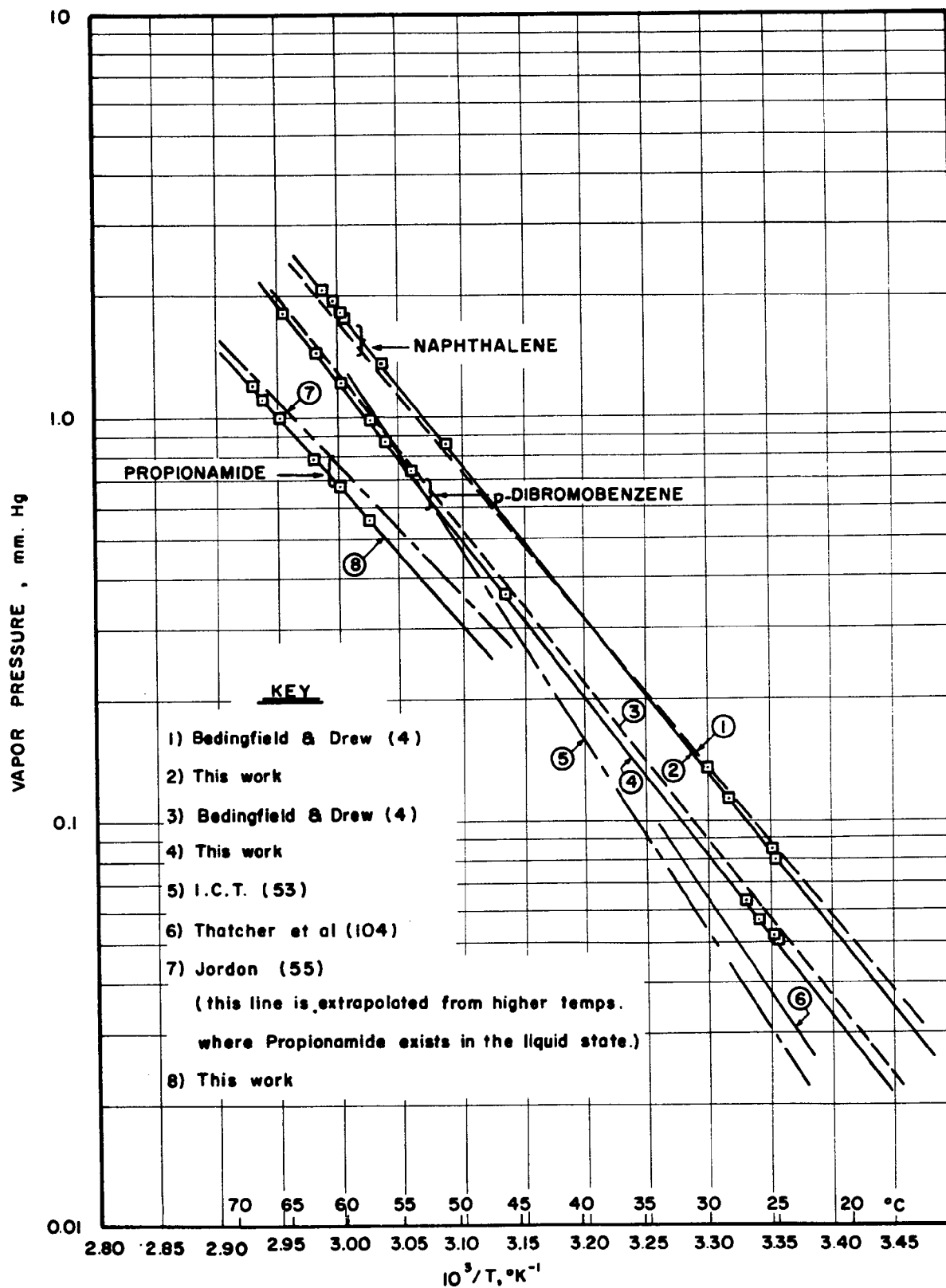
Figure 16a. Correlation of Vapor-Pressure Data for Naphthalene, p-Dibromobenzene, and Propionamide.
