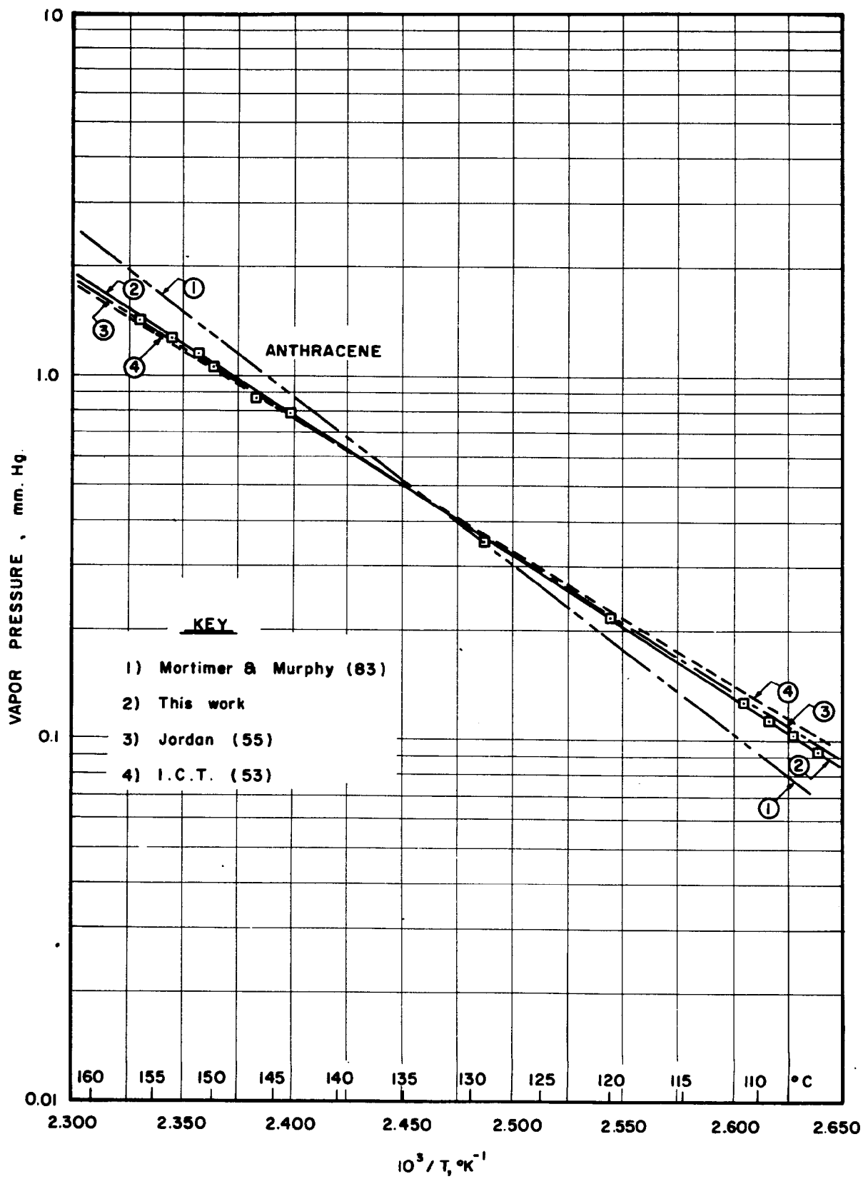
Figure 16b. Correlation of Vapor-Pressure Data for Anthracene.
