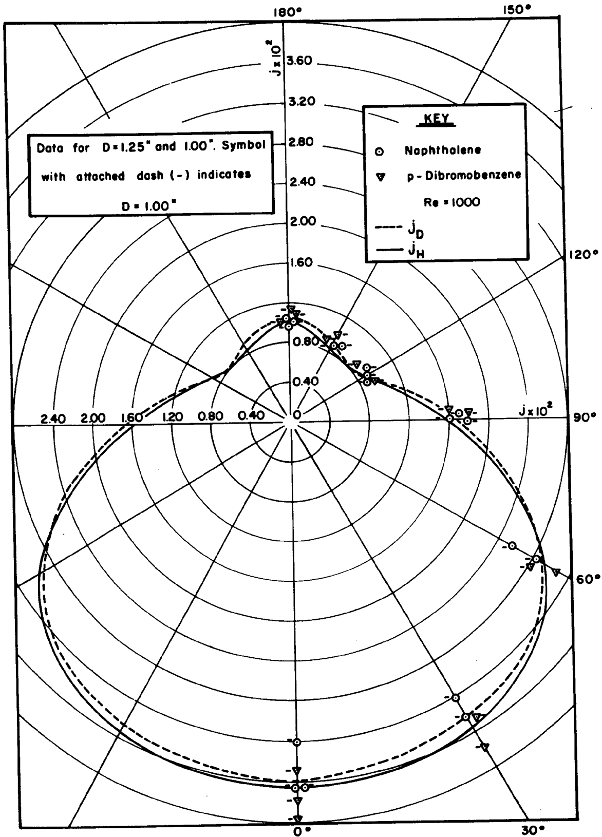
Figure 6b. Polar Diagrams for Heat and Mass-Transfer j -Factor Distributions at Re = 1000 . Data for \theta = 0^\circ, 30^\circ, 60^\circ, 90^\circ, 120^\circ, 150^\circ , and 180^\circ .
