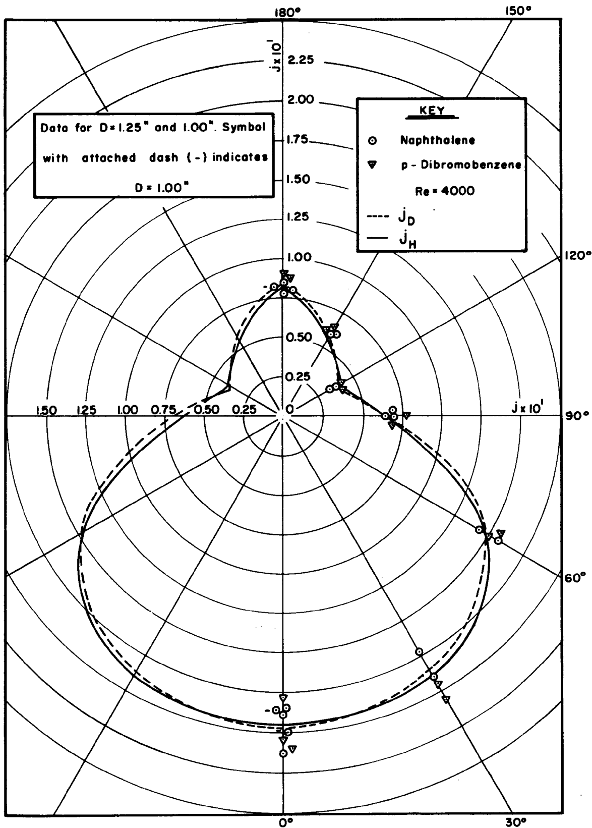
Figure 6d. Polar Diagrams for Heat and Mass-Transfer j -Factor Distributions at Re = 4000 . Data for \theta = 0^\circ, 30^\circ, 60^\circ, 90^\circ, 120^\circ, 150^\circ , and 180^\circ .
