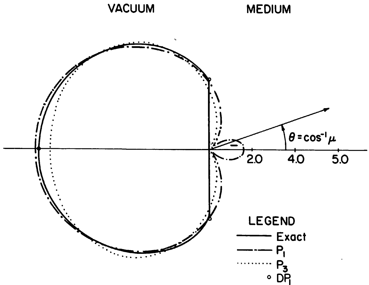
Fig. 8.4. Constant source angular distribution for Group 2, \psi_2(0, \theta) , Set I.
