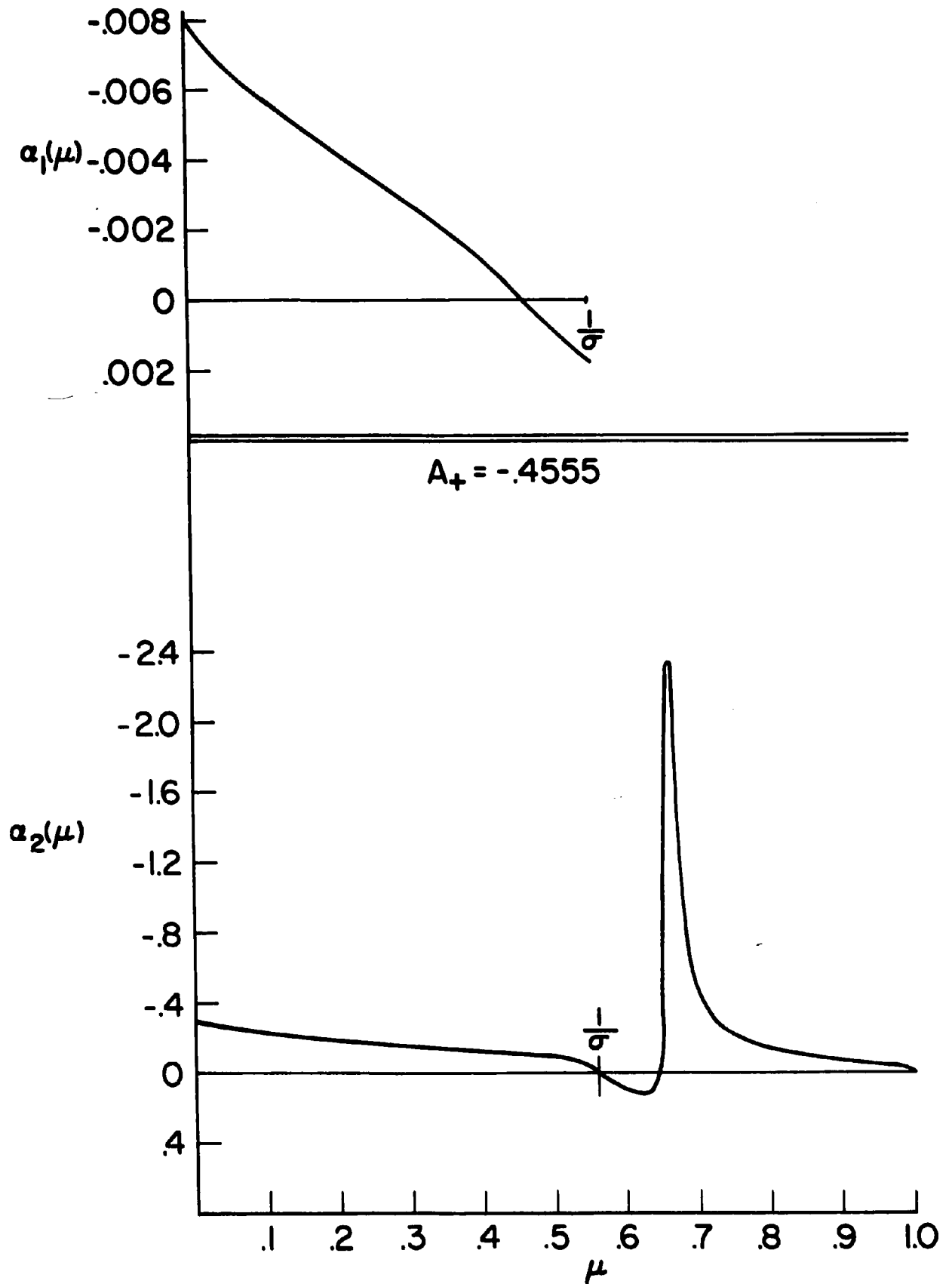
Fig. 8.2. Expansion coefficients for Milne problem, Set IV.
