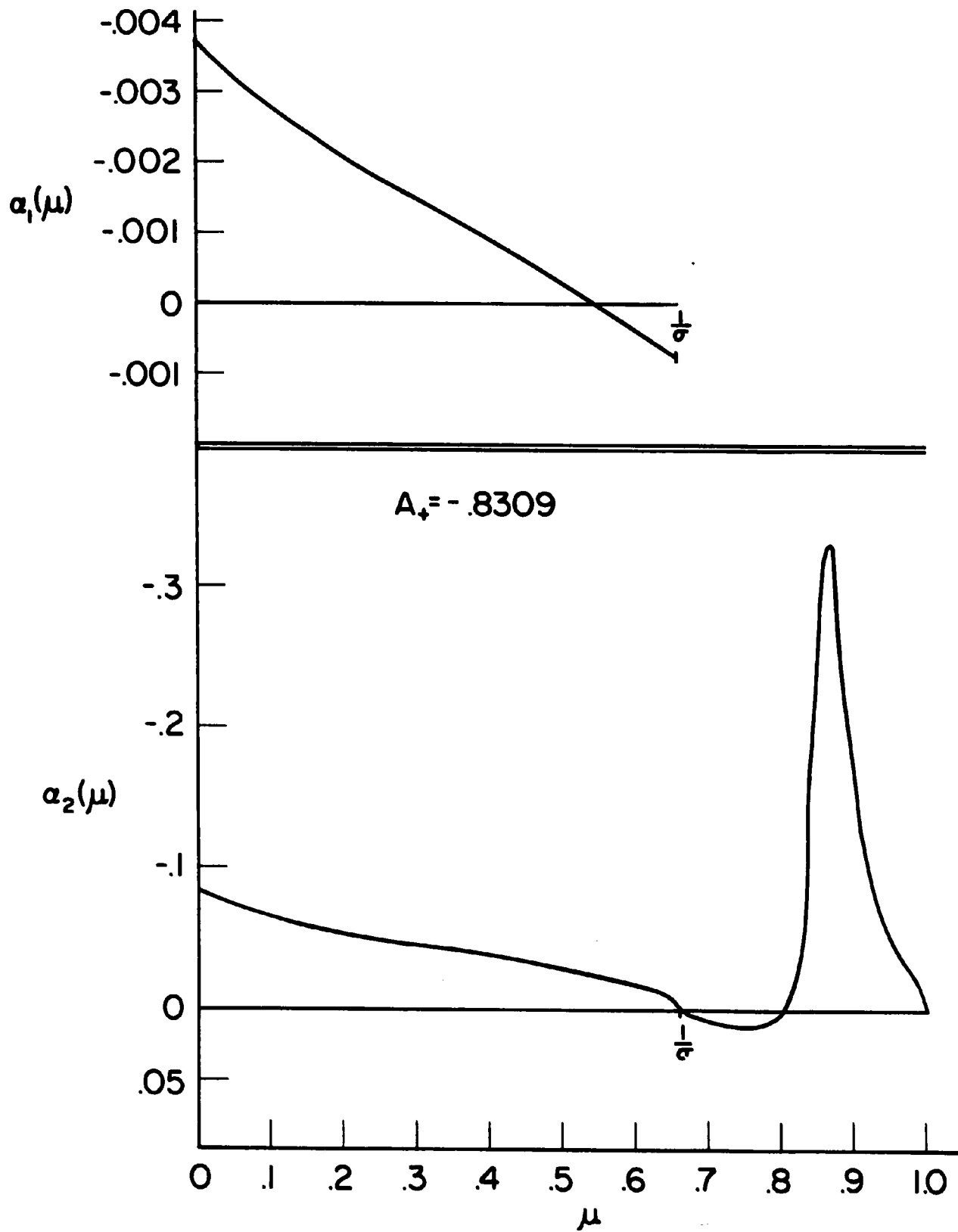
Fig. 8.1. Expansion coefficients for Milne problem, Set I.
