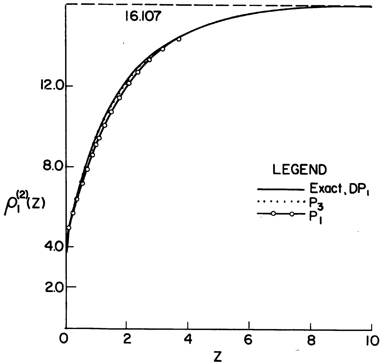
Fig. 8.9. Total flux for the constant source vs. distance into the medium, Group 2, Set IV.
