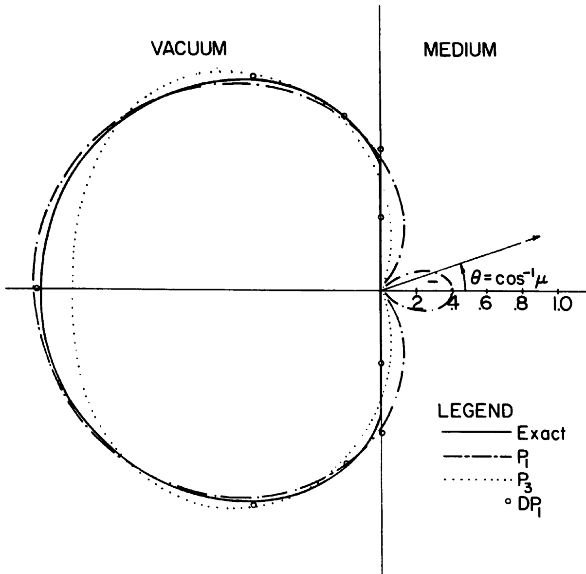
Fig. 8.3. Constant source angular distribution for Group 1, \psi_1(0, \theta) , Set I.
