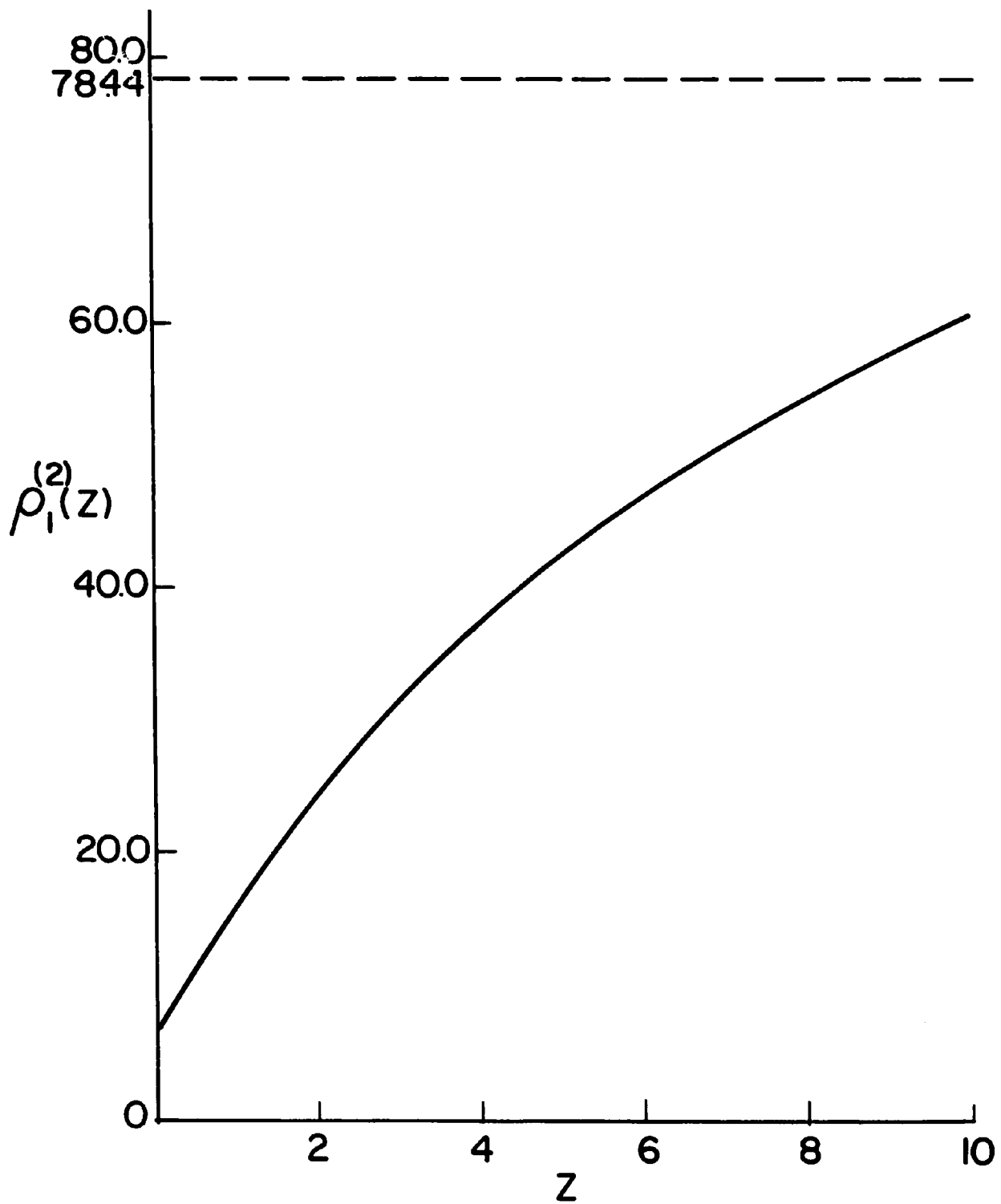
Fig. 8.8. Exact total flux for the constant source vs. distance into the medium, Group 2, Set I.
