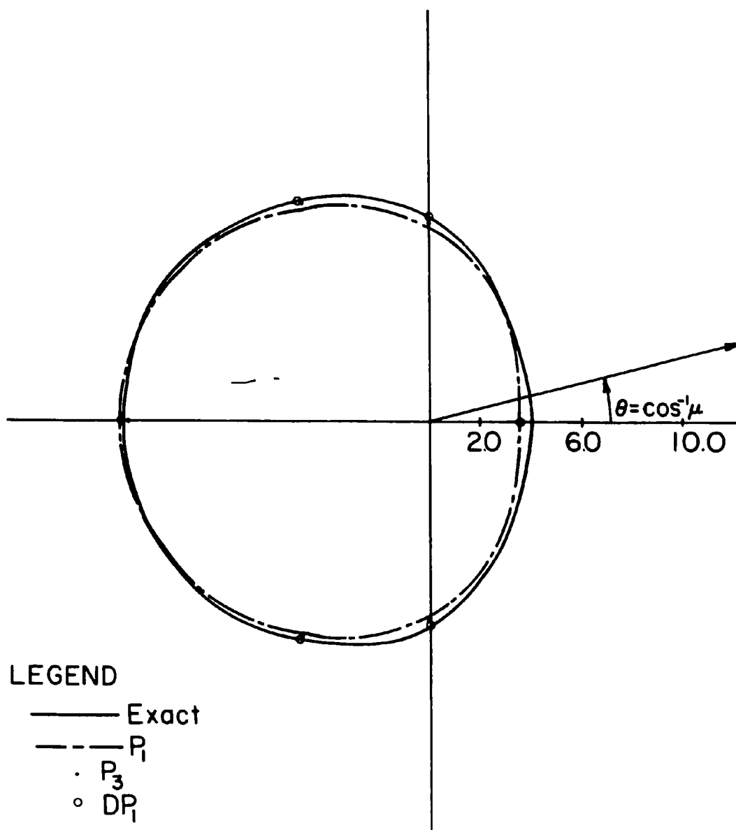
Fig. 8.5. Constant source angular distribution for Group 2, \psi_2(1, \theta) , Set I.
