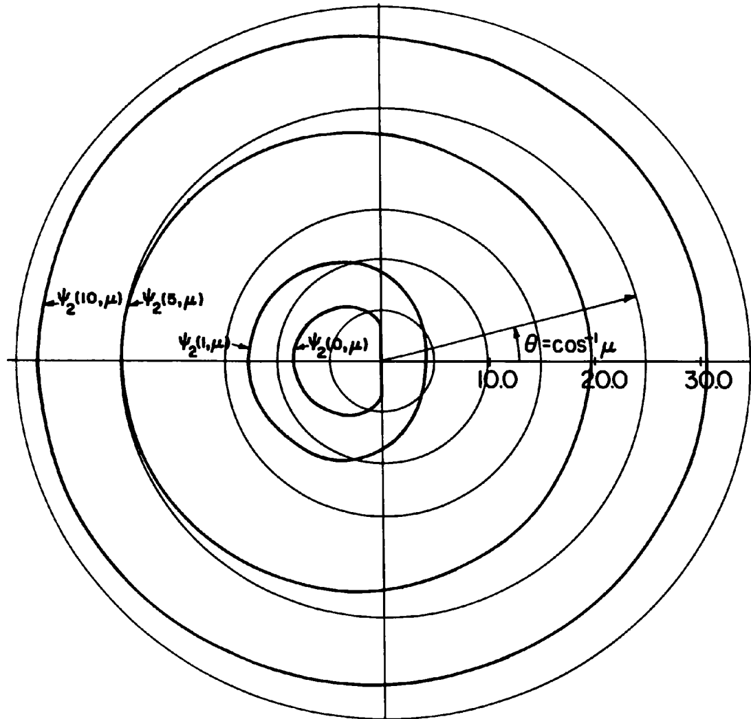
Fig. 8.6. Modifications in exact angular distribution with distance into the medium, Set I.
