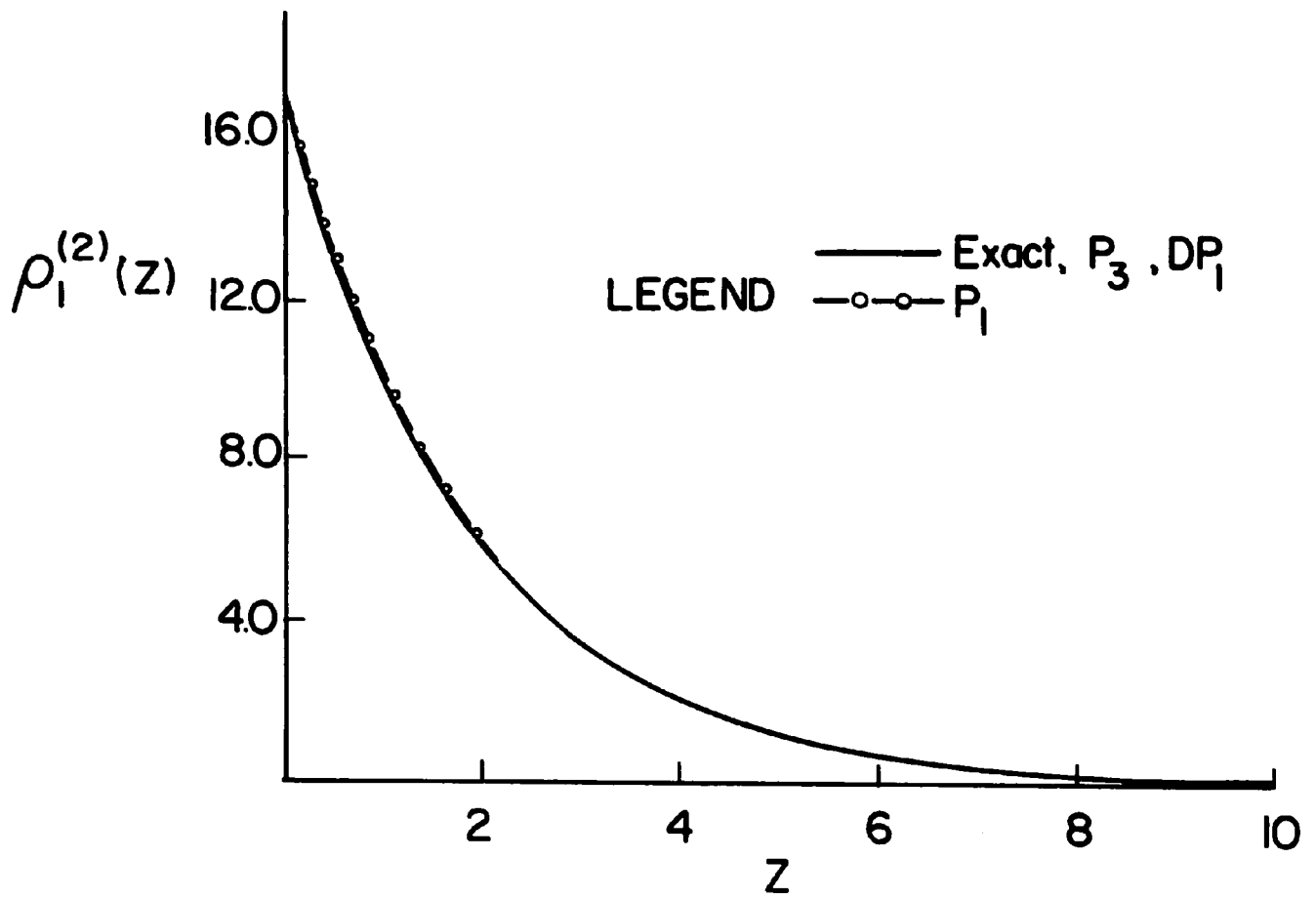
Fig. 8.10. Constant source current vs. distance for Group 2, Set IV.
