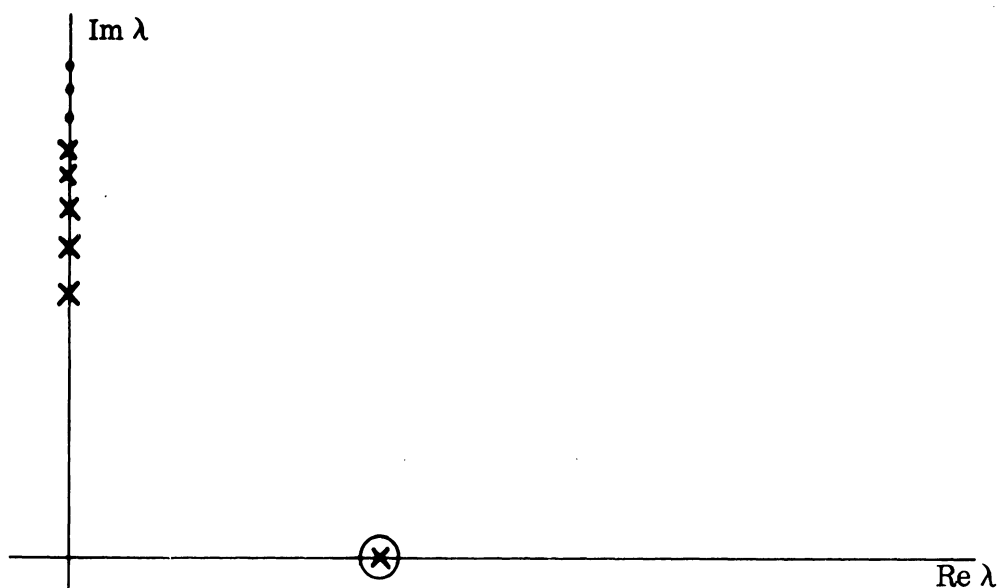
FIG. 4b: A SCHEMATIC REPRESENTATION OF THE POLES OF g_{\lambda}(r, r_0) WHEN \omega_b < |\omega| < \omega_c . The encircled pole is the gravity wave pole which lies in a different half plane from the others of the set.
