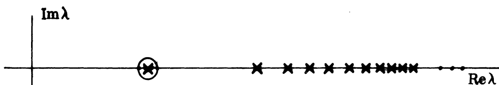
FIG. 4a: A SCHEMATIC REPRESENTATION OF THE POLES OF g_{\lambda}(r, r_0) WHEN |\omega| < \omega_b . The encircled pole is the gravity wave pole and lies in a different half plane from the others of the set.
