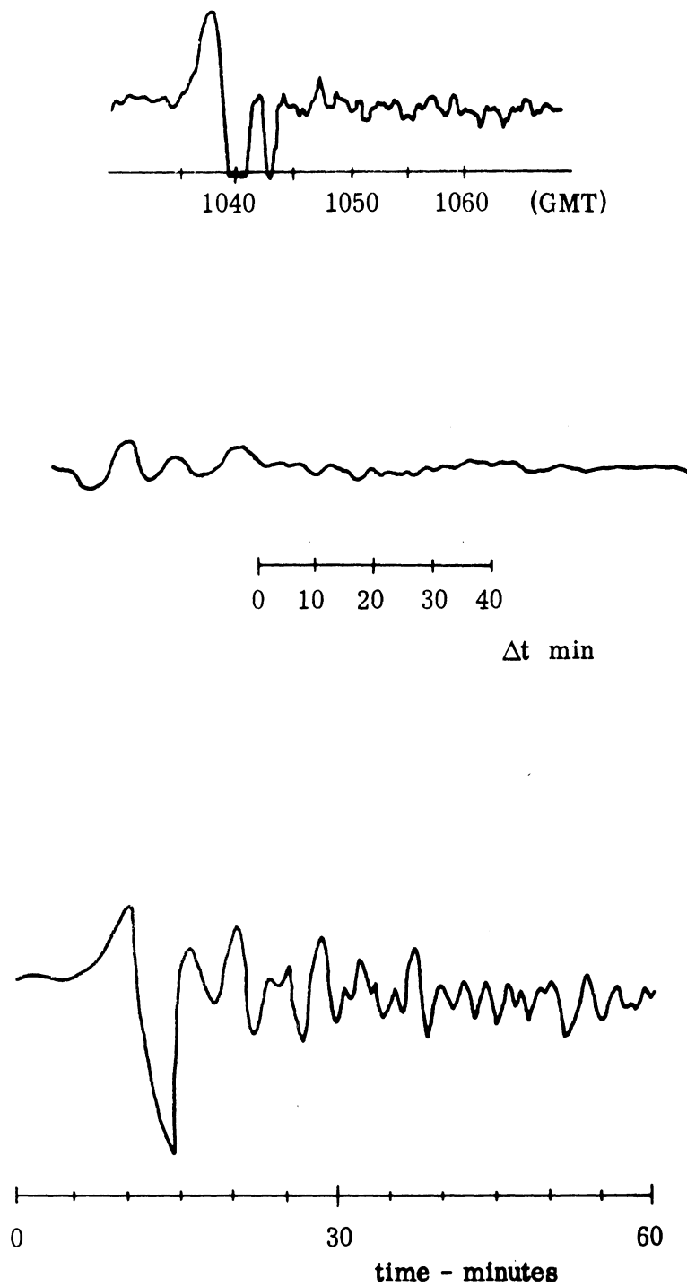
FIG. 8: SAMPLE MICROBAROGRAPH RECORDS. These data, from top to bottom were presented by Araskog, (19) Rose et al (23) and Donn and Ewing. (7)
