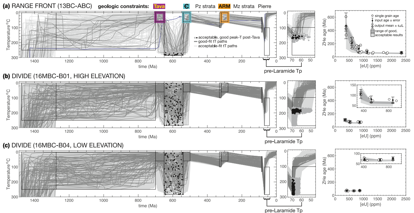
Figure 5. Combined thermal history modeling results; see Figure 3 for spatial location of geologic constraints highlighted in color. Black boxes define the parts of time-temperature ( tT ) space explored during each inversion; they are identical in these three inversions. The left panel presents the good- and acceptable tT paths. The right panel presents the corresponding fit to the ZHe age- [eU] trend. (a) The inversion result for the range front age- [eU] trend represented by samples 13BC-A, 13BC-B, and 13BC-C (Figure 4), from Murray, Stevens Goddard, et al. (2022, their Figure 6a). All good-fit and all but one acceptable-fit paths have late Neoproterozoic reheating with peak temperatures ( T_p ) of 240–285°C. The outlier acceptable-fit path (blue) is too hot for too long prior to Tava emplacement to be consistent with Mesoproterozoic biotite ^{40}\text{Ar}/^{39}\text{Ar} ages, which helps demonstrate the principal reasons Neoproterozoic heating is required (Murray, Stevens Goddard et al., 2022). Latest Cretaceous (i.e., pre-Laramide) peak temperatures are also tightly constrained by this result (middle panel). (b, c) The inversion results for divide samples (Figure 4), which do not resolve a particular Proterozoic history but do provide constraints on the pre-Laramide peak temperatures that are consistent with their relative elevations.
