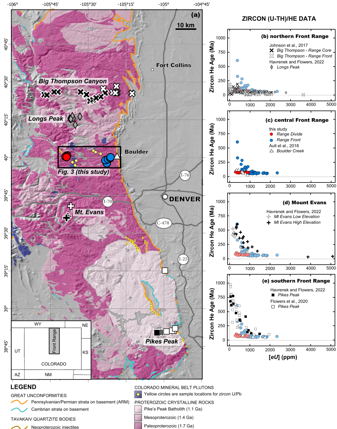
Figure 2. (a) A simplified geologic map of the crystalline rocks in the Front Range, the unconformable contacts between Proterozoic basement rocks and Cambrian (C) sediments or the late Paleozoic sediments deposited during the Ancestral Rocky Mountains (ARM) orogen (G. N. Green, 1992), and the Tavakaiv injectite localities (Cole & Braddock, 2009; Kellogg et al., 2008; Siddoway & Gehrels, 2014). Symbols indicate sample locations for this study (Murray, Niemi, & Clark, 2022), which are from the Paleoproterozoic basement rocks, and other published zircon (U-Th)/He (ZHe) thermochronology studies, which sampled a range of basement ages and lithologies. (b–e) ZHe data from the Front Range presented in age versus effective uranium concentration ([eU]) plots have a systematic relationship between age and grain U-Th composition that reflects the impact of radiation damage on the retention of ^4\text{He} in zircon (Guenther, 2021; Guenther et al., 2013). The data we interpret (red and blue circles) are presented on each panel to facilitate qualitative comparison among age-[eU] trends.
