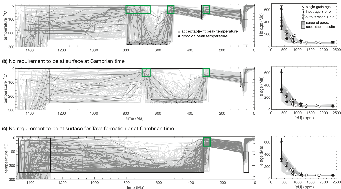
Figure 7. Inverse sensitivity tests using alternative translations of geologic observations into tT space (green tT boxes; Murray, Stevens Goddard, et al., 2022, their Figure 7). In each case, all good- and acceptable-fit paths are hot in Neoproterozoic–Paleozoic time but the timing of this heating, and the subsequent cooling, depends on the near-surface constraints. (a) Expanded Tava age constraint. (b) No requirement to be at the surface in Cambrian time. This result is also presented in Figure 6c, but here we zoom into Mesoproterozoic–Recent time and T < 300^{\circ}\text{C} . (c) No Proterozoic or Cambrian near-surface constraints.
