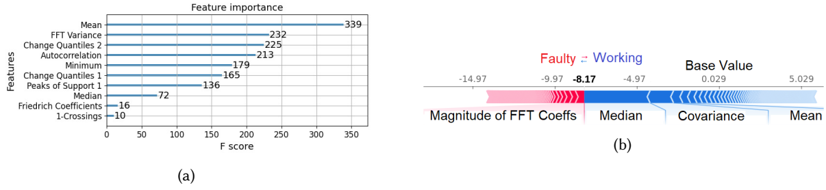
Fig. 9. (a) Top 10 features selected using B-H procedure, (b) Summary of Shapley Values showing FFT coefficients separate faulty and working classes.
