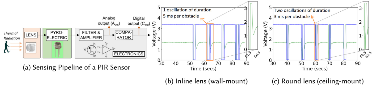
Fig. 3. Effect of different types of lens on the A_{out} curve, shown in green – the inline lens type produces a single oscillation whereas a round lens type produces two oscillation per obstacle. The corresponding C_{out} , shown in blue, stays HIGH when there is no motion and goes LOW when motion is detected.
