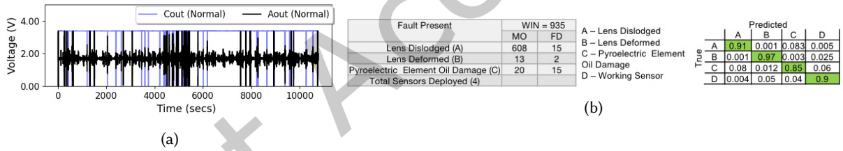
Fig. 17. Lobby Deployment (a) Occupancy graph during late evening from 6.45 pm to 9.45 pm at the lobby of our university building, (b) Deployment Statistics and confusion matrix of the classification model. Column titles: WIN →Total Number of Windows, MO →Misses Obstacle, FD → False Detection.
