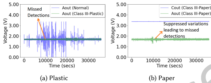
Fig. 7. Effect of different foreign particles producing Class III faults of different degree – the figures show that when the lens is obstructed with foreign particles like plastic tape and paper, it could result in complete failure.
