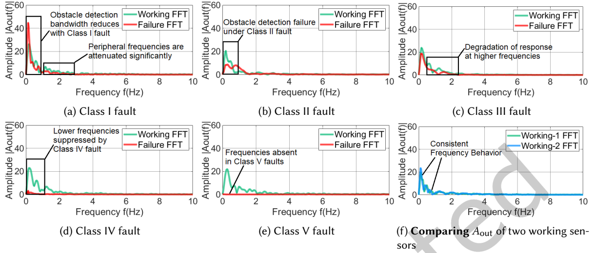
Fig. 8. Frequency Domain Representations of A_{out} under different faults in a PIR sensor. Only frequencies upto 10 Hz are shown as most PIR sensors detect human motion within 10 Hz.
