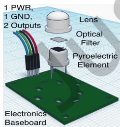
Fig. 2. PIR Sensor Teardown showing the different subsystems illustrated in TinkerCAD
