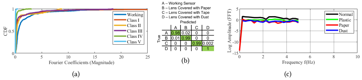
Fig. 23. (a) CDF of FFT Coefficients showing different distributions depending on the class of faults.,(b) Fine-grained Fault Analysis,(c) A_{out} waveforms showing different behavior for paper, plastic and dust obstructions.
