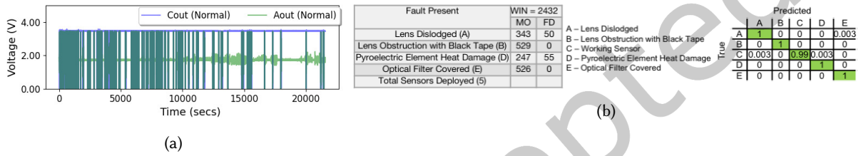
Fig. 16. Elevator Deployment (a) Occupancy : The graph is a 6 hour deployment during business hours, (b) Deployment Statistics and confusion matrix of the classification model. Column titles: WIN →Total Number of Windows, MO →Misses Obstacle, FD → False Detection.
