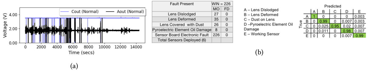
Fig. 18. Starbucks Deployment Occupancy : Evening deployment from 4.45 pm to 8.45 pm. The second half has much lesser little foot traffic. (b) Deployment Statistics and confusion matrix of the classification model. Column titles: WIN →Total Number of Windows, MO →Misses Obstacle, FD → False Detection.
