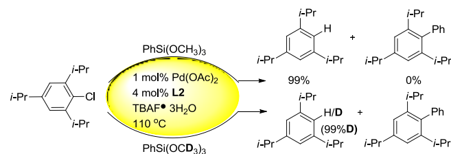
Scheme 1. Deuterium experiment of Hiyama coupling reaction of 1-chloro-2,4,6-triisopropylbenzene.
