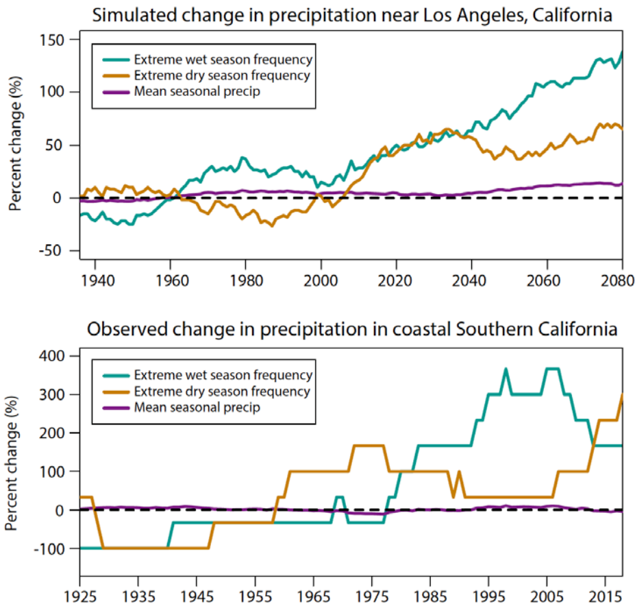
Figure 7. Simulated and observed changes in regional mean vs. extreme precipitation. a. Simulated change over time (across 40 ensemble members) in frequency of very wet (blue curve) and very dry (brown curve) November-March "rainy seasons"—as well as the relative change in mean seasonal precipitation (purple curve)—for a grid box near Los Angeles, California as simulated in the CESM Large Ensemble experiment (CESM-LENS) under an RCP 8.5 greenhouse gas emission scenario. b. Same as a., but using observed precipitation for California's "South Coast Drainage" (which encompasses Los
