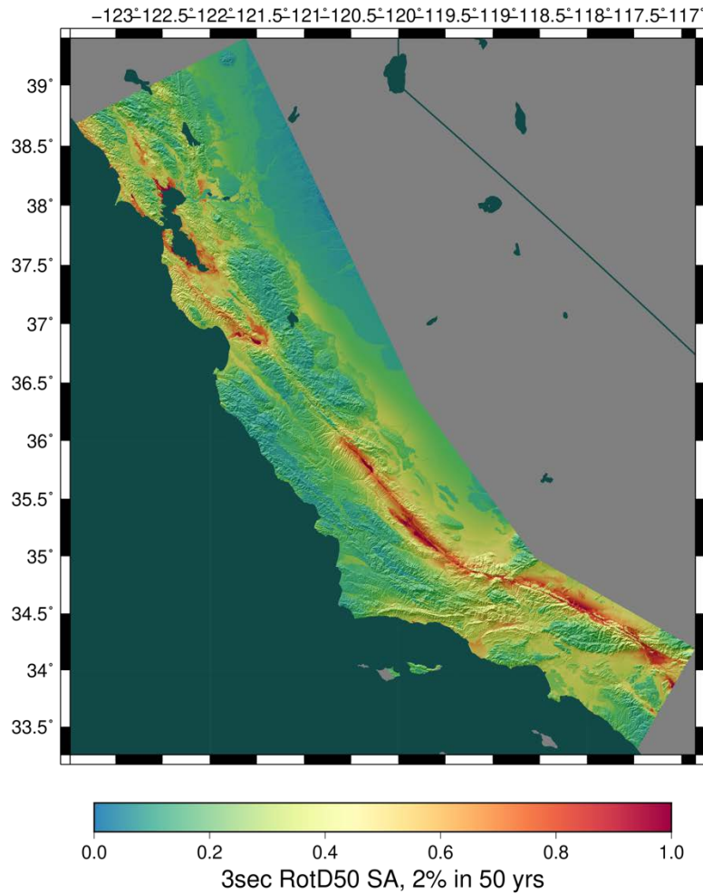
Figure 5. CyberShake map for 0.33 Hz (3s) spectral acceleration for 2% in 50 years probability of exceedance. The composite map was produced by combining the 3D southern California map (Study 15.4), the central California map (Study 17.3), and the northern California map (Study 18.8). . In aggregate, the combined map includes 650 million seismograms representing ground motions at 1,673 sites; it took over 175 million core-hours of processing time to complete using NCSA Blue Waters and OLCF Titan, the two largest open-science supercomputers available at the time.
