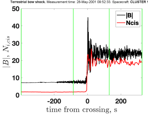
Figure 4. Example of a plot of the terrestrial bow shock, measured by CLUSTER CS1. Shown are the magnetic field magnitude and the CIS measured ion density. The vertical green lines denote the chosen upstream and downstream regions used in the analysis.
